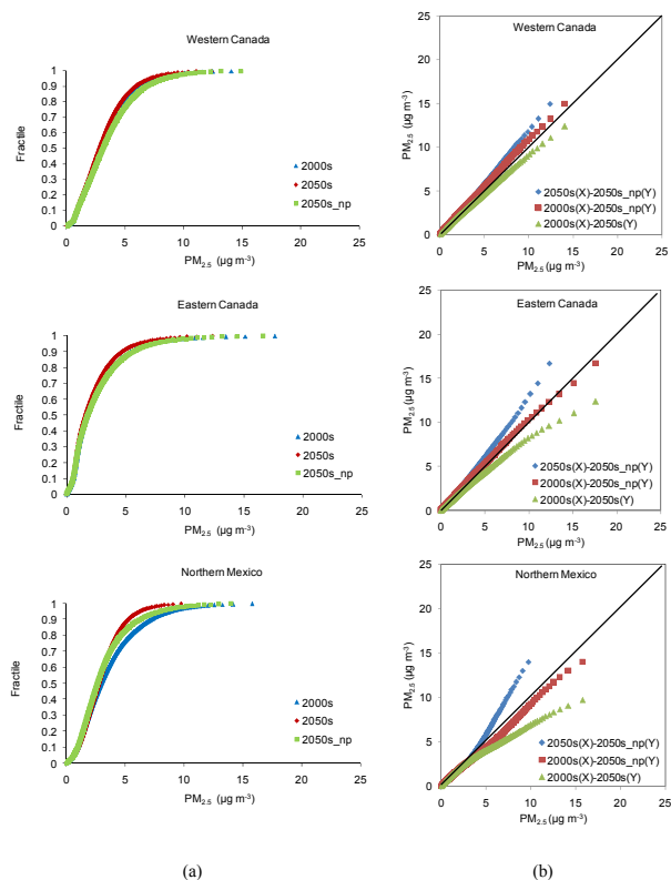
Fig. 7. Daily average PM_{2.5} concentration cumulative distribution function (CDF) plots (a) for historic and future summers and the correlation (b) between the different examined cases. (np: 2001 emission inventory and 2050 meteorology).
