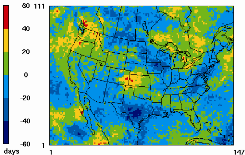
Fig. 2b. Spatial distribution plots for the change in rainy days between the three historic and future summers.
