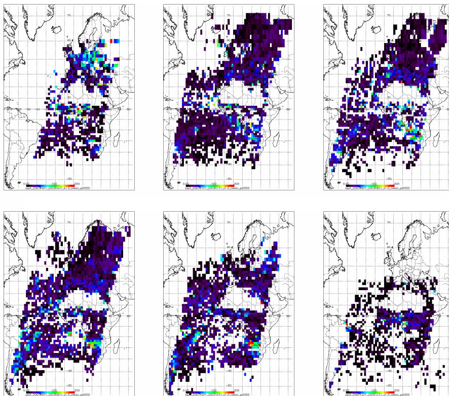
Fig. 11. Seasonal variation of soot: Monthly average AOD on a 5^{\circ} \times 5^{\circ} grid of the soot component for the months April, July, August, September, October 2003, and December 2005 are shown from left to right/top to bottom.
