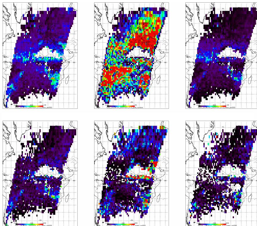
Fig. 10. Examples of a 4-monthly average map based on SYNAER data of July–October 2003 on a 5^{\circ} \times 5^{\circ} grid: upper line from left to right: total AOD at 550 nm, the number of contributing pixels per box, and component AOD at 550 nm of water-soluble aerosols; lower line from left to right: component AOD at 550 nm of soot, mineral, and sea salt aerosols. Note the different colour bars ranging from 0–50 for pixel number, from 0.0 to 1.0 for total and water-soluble AOD, and from 0.0 to 0.2 for components in the lower line.
