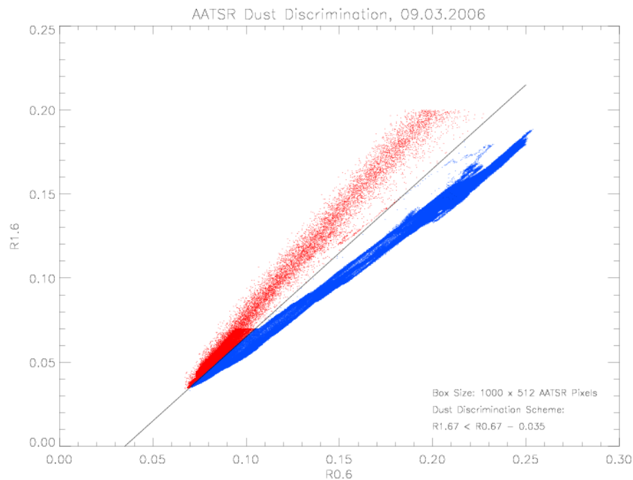
Fig. 4. Scatter plot of AATSR reflectances at 1.6\ \mu\text{m} against 0.6\ \mu\text{m} for a scene from 9 March 2006 showing the differentiation of heavy dust load and shallow stratocumulus clouds.
