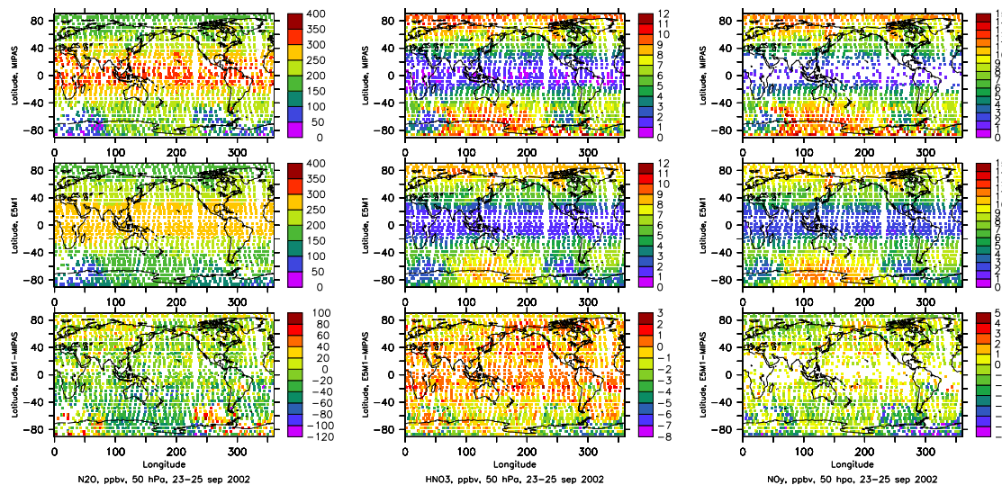
Fig. 3. N 2 O, HNO 3 , NO y (first 3 rows), NO 2 , N 2 O 5 , NO (second 3 rows), O 3 , ClONO 2 (ClONO 3 ) and HNO 4 (third 3 rows) at 50hPa for 23–25 September 2002 as observed by MIPAS (upper panels of each group), simulated by ECHAM5/MESy1 (middle panels) and deviations of the model to MIPAS (point-by-point in space and time, lower panels of each group).
