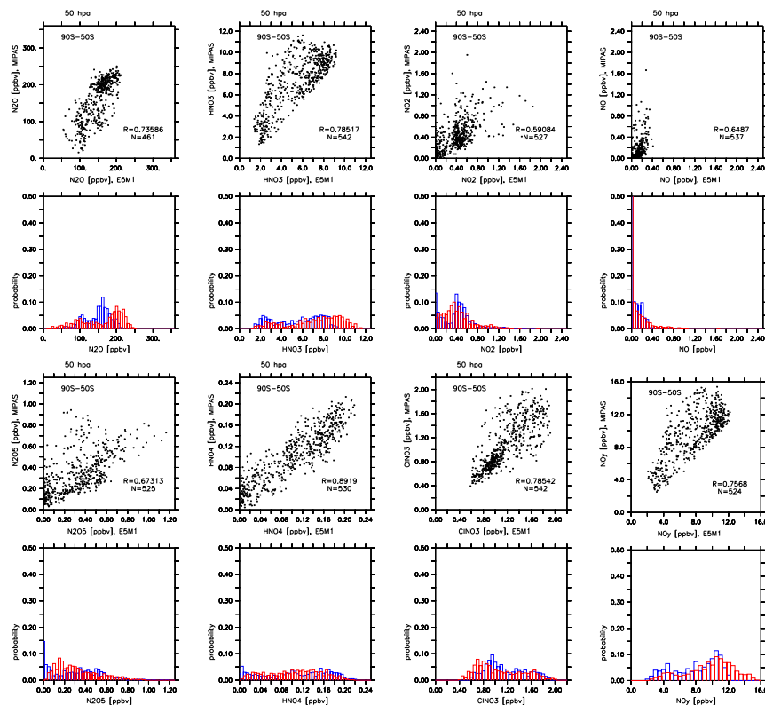
Fig. 5. Point-by-point correlations of MIPAS data to ECHAM5/MESSy results and probability density functions (PDF) for 50 to 90° S at 50 hPa, 23–25 September 2002. MIPAS red, model blue. Upper rows: N 2 O, HNO 3 , NO 2 , NO; lower rows: N 2 O 5 , HNO 4 , ClONO 2 and total nitrogen NO y . R is the correlation coefficient, N the number of data points in the latitude bin. For the PDFs the bins for the observations are shifted by 10% of the binsize for better visibility.
