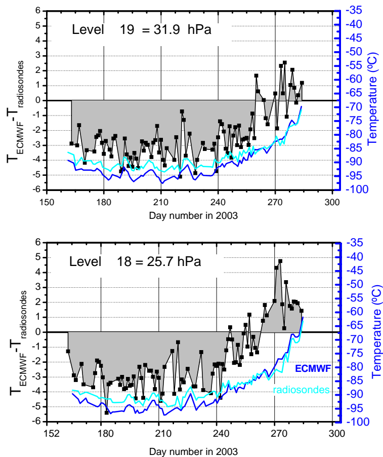
Fig. 2. Evolution of temperatures during the winter 2003 for radiosondes and EMCWF model at the lower stratosphere representative levels of 31.9 and 25.7 hPa (right axis) and \Delta T (left axis) above Belgrano.
