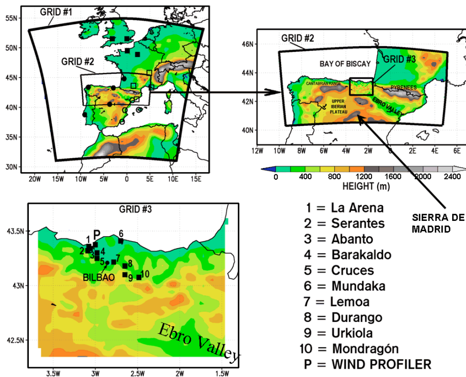
Fig. 1. Topographic map of the three domains (grid 1, 2 and 3) used by RAMS and HYPACT. (Top-left) The European pollution sources selected for the simulations are represented with closed squares and circles (regions A and B, respectively), and open squares and circles (regions C and D). (Bottom-left) The Basque Country is completely included in grid 3, where the upper Ebro valley, the location of the WPR (marked P) and the selected ozone monitors (1-to-10) have also been represented. (Top-right) Main topographic features surrounding the Basque Country are represented in the intermediate grid #2, and (bottom-right) the list of the ozone stations.
