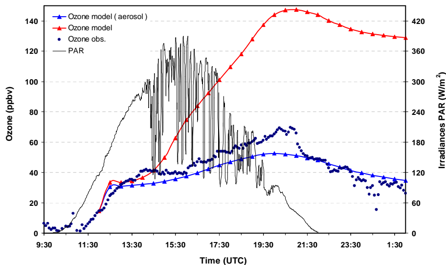
Fig. 11. O_3 observed at surface on 19 September 2002 at Fazenda N. Senhora site and the comparison with modeled O_3 by the OZIPR model including (blue line) and neglecting (red line) the aerosol load concentration. The measured PAR surface irradiances ( Wm^{-2} ) are also shown to track the diurnal solar cycle.
