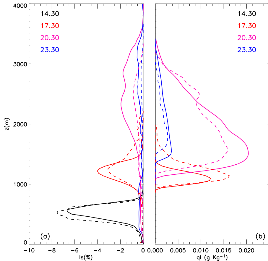
Fig. 13. Time evolution of the vertical profile (one-hour slab averaged) of the (a) intensity of segregation of species B and C and of the (b) liquid water content. WUR-LES: solid line and NCAR-LES dashed line.
