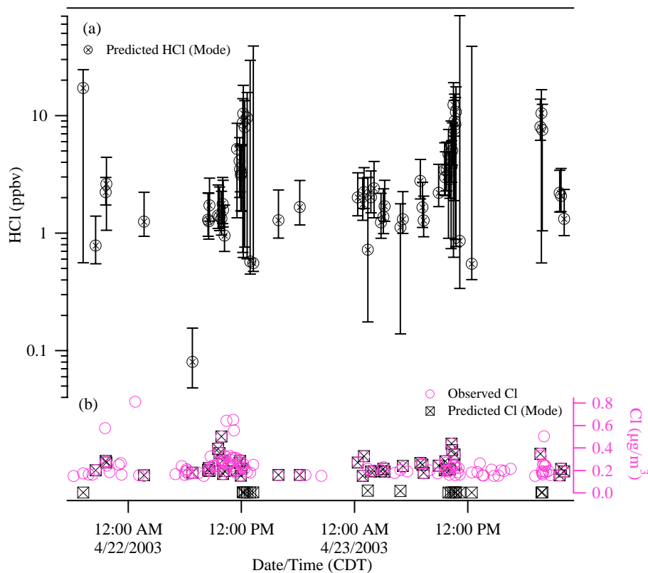
Fig. 12. (a) Posterior distribution of HCl(g) concentrations on 22–23 April at Pedregal. The points represent the mode of the probability density function and the error bars are the 95% confidence intervals. Only points whose Markov Chain passed the convergence tests described in Part I are included. (b) Predicted (mode) and observed aerosol chloride concentrations, where only the observations above the detection limit are shown. The model was not run if the ammonia observations were lacking, even when the observed aerosol chloride concentration was above the detection limit.
