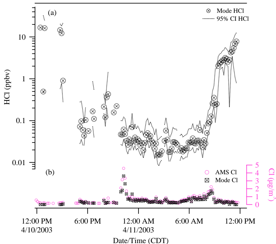
Fig. 8. (a) Posterior distribution of HCl(g) concentrations on 10–11 April at CENICA. The points represent the mode of the probability density function and the dashed lines are the 95% confidence intervals. Only points whose Markov Chain passed the convergence tests described in Part I are shown. (b) Predicted (mode) and observed aerosol chloride concentrations, where only the observations above the detection limit are shown. The aerosols are assumed to be stable; note that the aerosols are assumed to effloresce at 16:30 on 10 April and deliquesce at 09:30 on 11 April.
