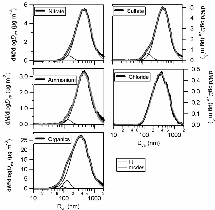
Fig. 7. Results of the multimode lognormal fits performed to the size distributions of the NR-PM 1 components. In each plot the lognormal modes resulting from the fit are shown. The sum of the modes is plotted in grey, while the data is plotted in thick black.
