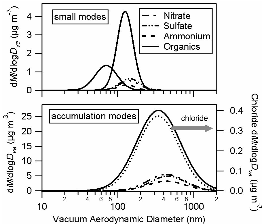
Fig. 8. “Small” and “accumulation” modes of the NR-PM 1 species as calculated from the multi-mode lognormal fits.
