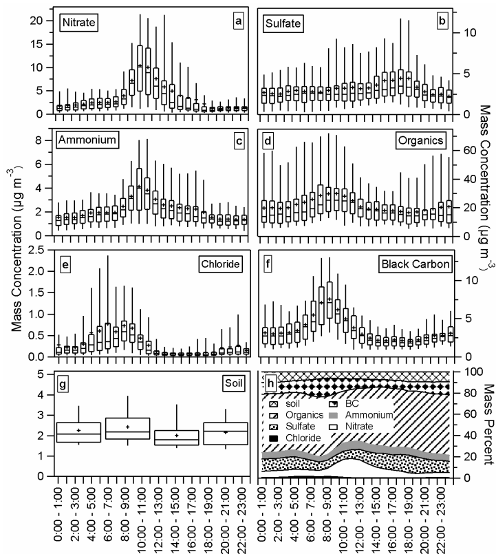
Fig. 4. Panels (a)–(g): box-whisker plots of the diurnal cycles of the mass concentration of particulate species. Crosses represent the average mass concentration; horizontal lines represent the median; bottom and top of the boxes represent the 25 and 75% limits respectively; and the bottom and the top whiskers represent the 5 and 95% limits respectively. Averages are made over the complete time interval where data is available. Panel (h): Diurnal cycle of the fractional mass concentration of various aerosol species to \text{PM}_{2.5} . Average was made over the time interval where AMS, BC, and soil data are available (see Fig. 3).
