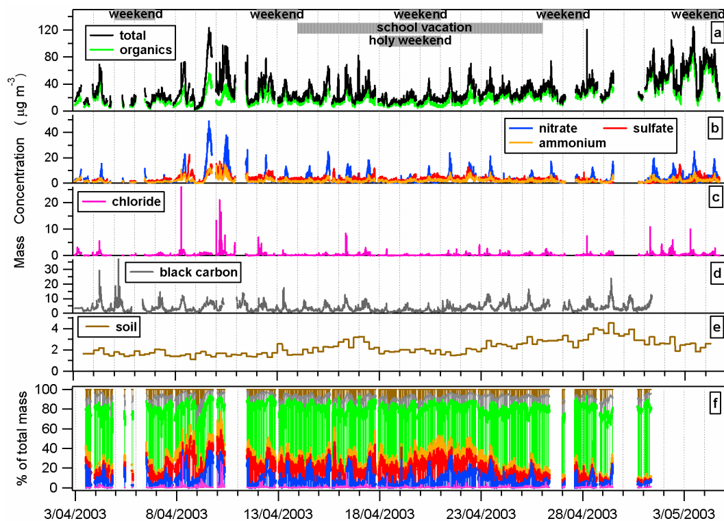
Fig. 3. Panels (a)–(e). Time series of the mass concentration of the AMS NR-PM 1 species (Total = nitrate + sulfate + ammonium + chloride + organics), aethalometer BC, and estimated soil at the CENICA Supersite. Panel (f): Time series of the percent mass composition of Total AMS + BC + soil.
