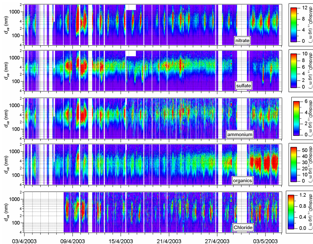
Fig. 5. Image plots of the mass concentration of the main NR-PM 1 species as a function of time and size for all of MCMA-2003.
