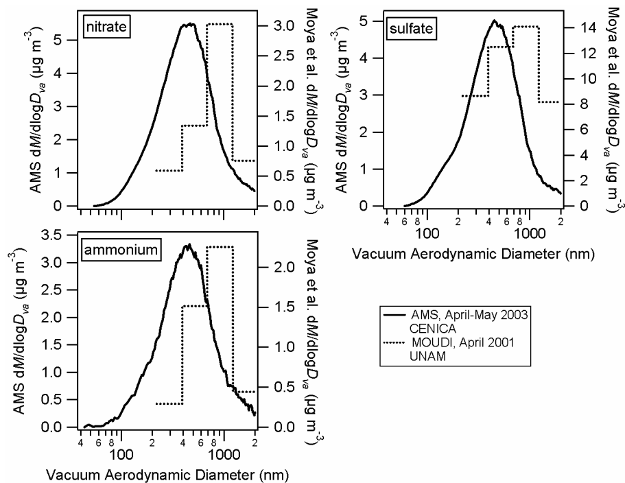
Fig. 12. Size distributions of the main inorganic components of the Mexico City aerosol measured with the AMS at CENICA during the MCMA-2003 in April–May 2003; and by Moya et al. (2003), measured with a MOUDI in the main campus of UNAM in April 2001. Note the different scales for both datasets.
