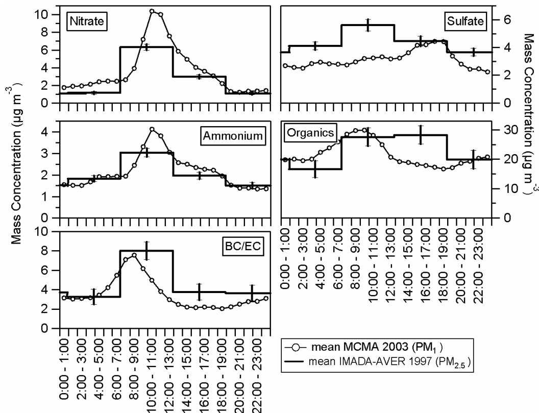
Fig. 9. Average diurnal profiles of PM_{2.5} species measured during IMADA-AVER at CES in February–March 1997 (Chow et al., 2002) and during MCMA-2003. All data is plotted vs. local time. Soil diurnal cycles are not compared because Chow et al. (2002) only report 24-h average concentrations for particle metals.
