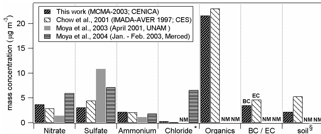
Fig. 11. Comparison of the average mass concentrations of some PM_{2.5} species reported for Mexico City by the authors at CENICA during MCMA-2003 in April–May 2003; by Chow et al. during IMADA-AVER at CES in February–March 1997 (Chow et al., 2002); by Moya et al. (2003), at the main campus of UNAM in April 2001 ( 0.18\text{--}1.8\ \mu\text{m}\ d_{va} ); and by Moya et al. (2004) at Merced in January–February 2003 ( 0.18\text{--}1.8\ \mu\text{m}\ d_{va} ). NM = no measurement available.
