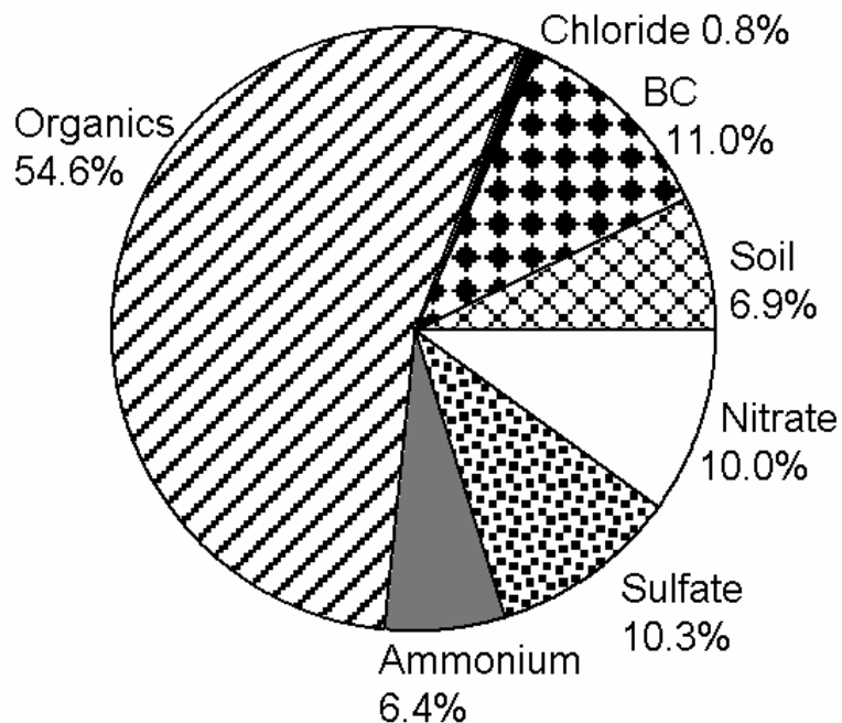
Fig. 2. Average mass composition of PM_{2.5} (approximated as AMS + BC + soil) for the MCMA-2003 campaign. Average was made over all time periods where data from the three measurements were available.
