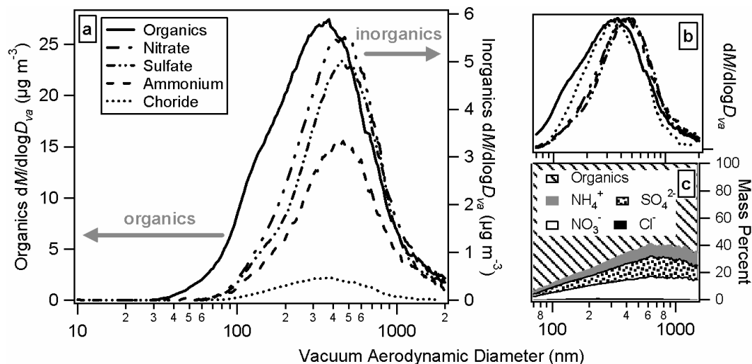
Fig. 6. Panel (a): Average size distributions of NR-PM 1 species for the entire measuring period. Panel (b): size distributions normalized to the same maximum so that their relative shapes can be appreciated. Panel (c): percent concentration of the total NR-PM 1 mass as a function of particle size. Note the different axis scales in which the inorganic and organic distributions are plotted in panel (a).
