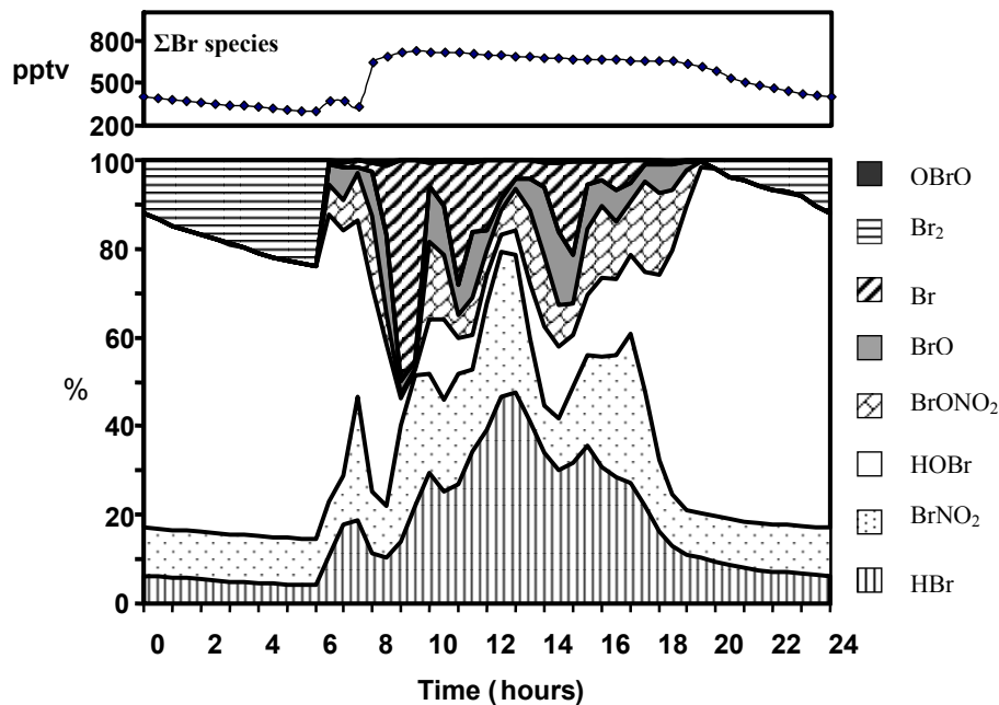
Fig. 6. Cumulative diurnal profile of significant bromine species. “ \Sigma\text{Br species} ” refers to the sum of the 8 bromine species shown in the lower panel.
