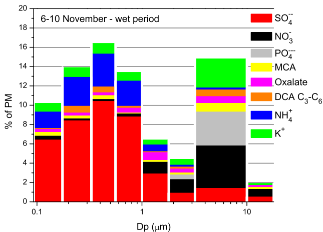
Fig. 7. Ionic mass fraction as a function of the particle aerodynamic diameter in MOUDI samples collected in FNS, Rondônia, Brazil, 2002: (a) MDRO37; (b) MDRO60b.
