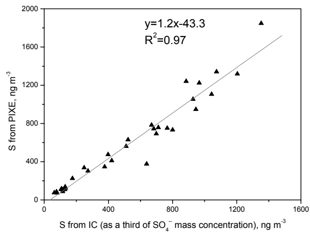
Fig. 5. Comparison between Sulfur (a) and Potassium (b) mass concentrations measured by PIXE and by ion chromatography in samples collected in FNS, Rondônia, Brazil, 2002.
