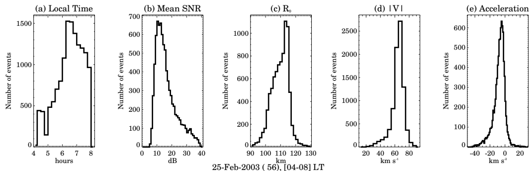
Fig. 6. Meteor statistics similar to Fig. 5 during a control day (when Leonid shower was not present) of 25 February 2003.
