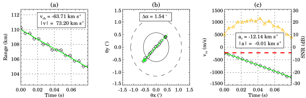
Fig. 3. Meteor characterization for most meteor events. (a) Range vs. time, (b) \theta_x vs. \theta_y , and (c) pulse-to-pulse Doppler vs. time. In all three cases the fitting lines are represented in green. In panel (c) the SNR is shown along the meteor trajectory (scale on the right) in orange, while the absolute acceleration is given by the slope of the red line.
