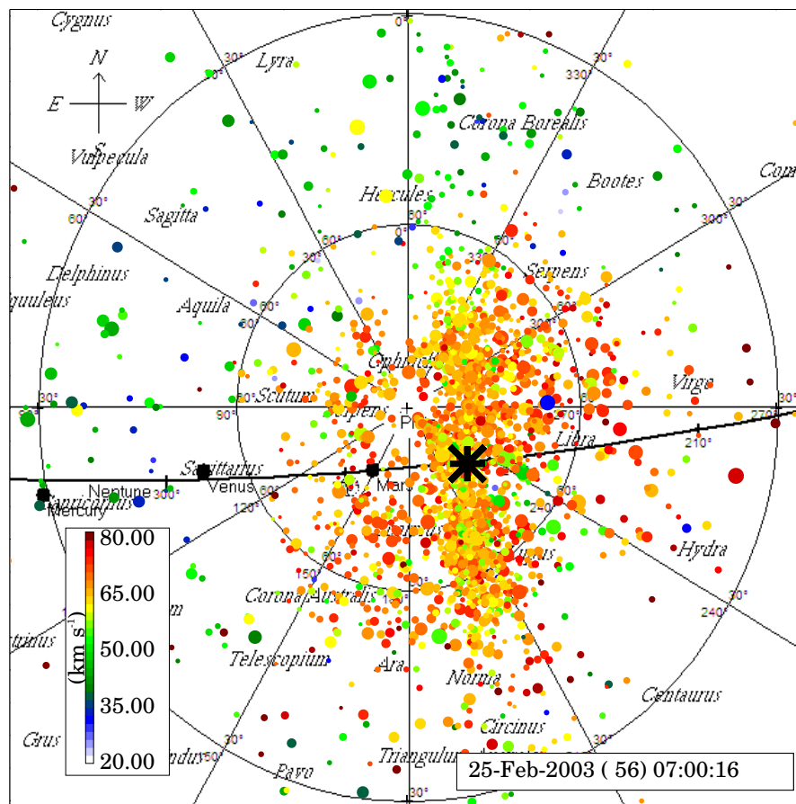
Fig. 9. Skymap distribution of meteors similar to Fig. 7 but for a control day around 07:00 LT on 25 February 2003.
