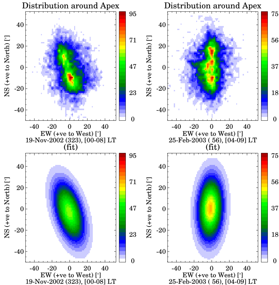
Fig. 10. Angular velocity distribution of meteors around the Apex for the Leonid night (left) and control day (right). Bottom panels show the fitted distributions using two-dimensional Gaussian functions.
