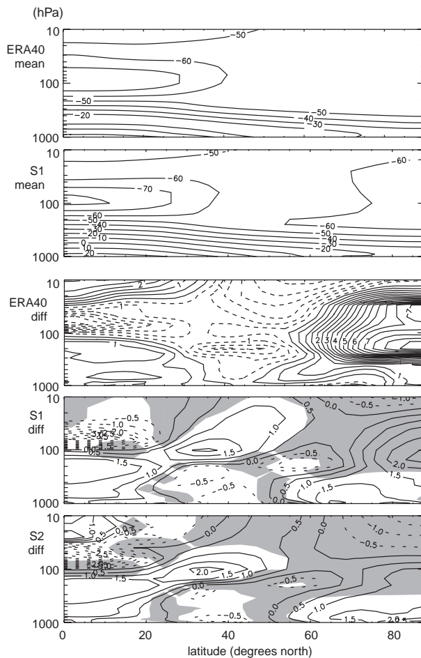
Fig. 6. Mean value and difference between 1987 and 1989 in zonal mean temperature (°C), averaged from January to March, in ERA40, S1, and S2. Shaded areas are not significantly different from zero (t-test, p < 0.05 ).
