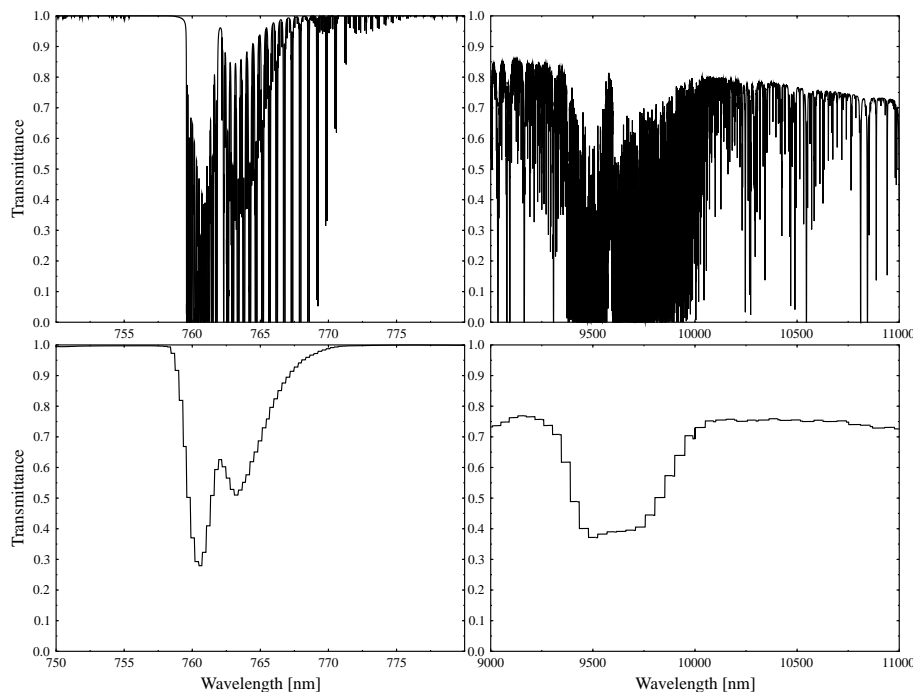
Fig. 3. uvspec direct transmittance in the O 2 A-band around 760 nm (left) and in the IR window region (right), for the midlatitude summer atmosphere of Anderson et al. (1986) . (Top) line-by-line calculation, based on spectral absorption cross sections provided by genln2; (bottom) pseudo-spectral calculation, based on the LOWTRAN absorption parameterization.
