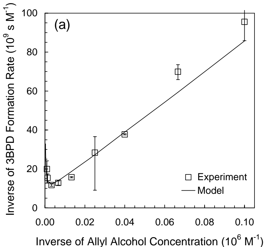
Fig. 6. (a) Inverse plot for the competition kinetics experiment 1 described in Table 1 and Fig. 5a ( [\text{Br}^-]=0.80 \text{ mM} , pH 5.3). The squares are the inverse of the experimentally determined rates of 3BPD formation and the line shows the corresponding results from the \text{Br}^- Full Model. Error bars represent 90% confidence intervals around the experimental data.
