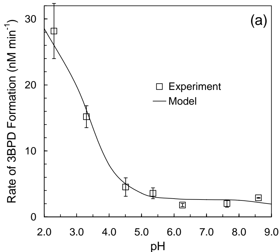
Fig. 4. (a) Rate of 3-bromo-1,2-propanediol (3BPD) formation ( R_{F,tot}^{3BPD} ) as a function of pH in illuminated (313 nm) aqueous bromide solutions ( [\text{Br}^-]=8.0 \text{ mM} ) containing 1.0 \text{ mM H}_2\text{O}_2 and 75 \mu\text{M AA} . The squares are experimental values of R_{F,tot}^{3BPD} . Error bars for 3BPD represent the 90% confidence interval for each point, calculated from the standard error of the slope from plots of 3BPD versus time at each pH. The line is the result from the "Br - Full Model".
