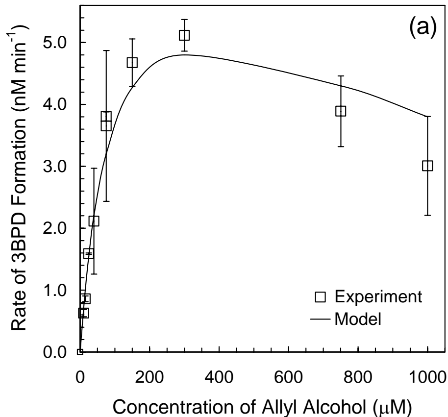
Fig. 5. (a) Experimental and model values of the total rate of 3-bromo-1,2-propanediol (3BPD) formation ( R_{F,\text{tot}}^{3\text{BPD}} ) for competition kinetics Experiment 1 (pH 5.3, 0.80 mM Br - , 1.0 mM H 2 O 2 , 10–1000 μM AA, 313 nm illumination). Symbols, line, and error bars are the same as in Fig. 4a.
