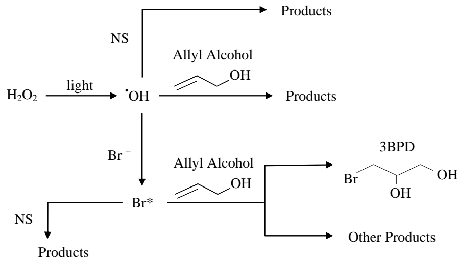
Fig. 1. (a) Simplified scheme showing the formation of reactive bromine species ( \text{Br}^* ) and their reaction with allyl alcohol (AA) to form 3-bromo-1,2-propanediol (3BPD). Note that AA also consumes \cdot\text{OH} , thereby decreasing the rates of formation of \text{Br}^*(\text{aq}) and 3BPD (i.e., the “AA effect”). NS=natural scavengers, i.e., other sinks for \cdot\text{OH} and \text{Br}^*(\text{aq}) .
