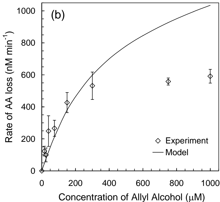
Fig. 5. (b) Experimental and model values of the rate of allyl alcohol loss ( R_L^{\text{AA}} ) as a function of allyl alcohol concentration for competition kinetics experiment 1 presented in Fig. 5a and Table 1. The symbols, line, and error bars are the same as described in Fig. 3.
