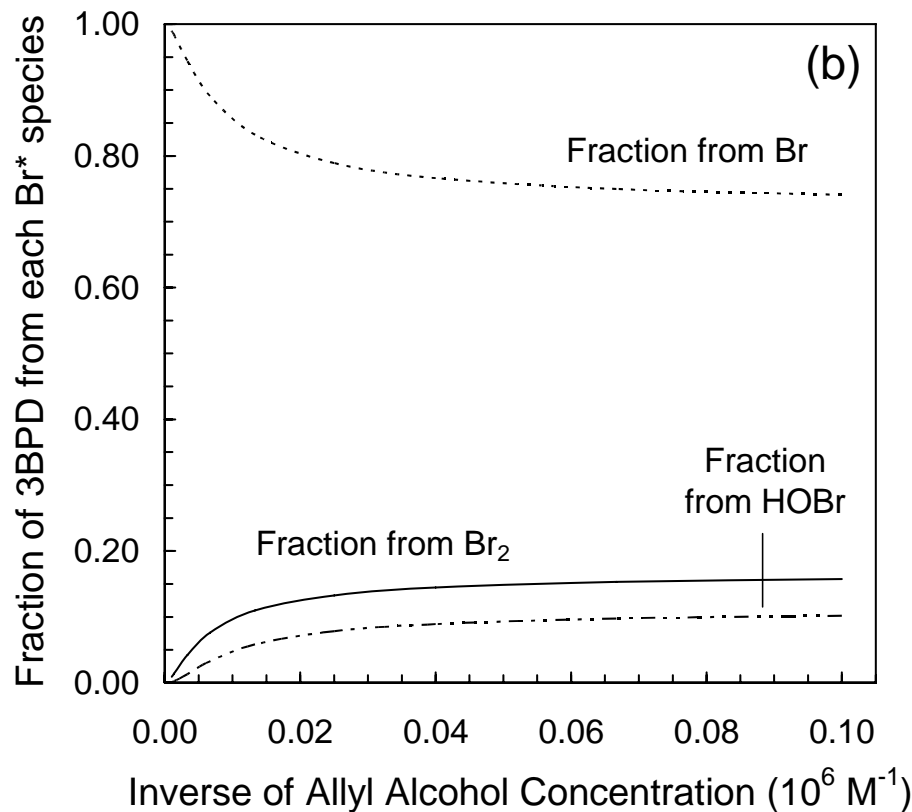
Fig. 6. (b) The fractions of 3BPD formed from the reaction of species i with AA ( F_i^{3\text{BPD}} ) as a function of 1/[\text{AA}] for competition kinetics experiment 1 in Fig. 6a.
