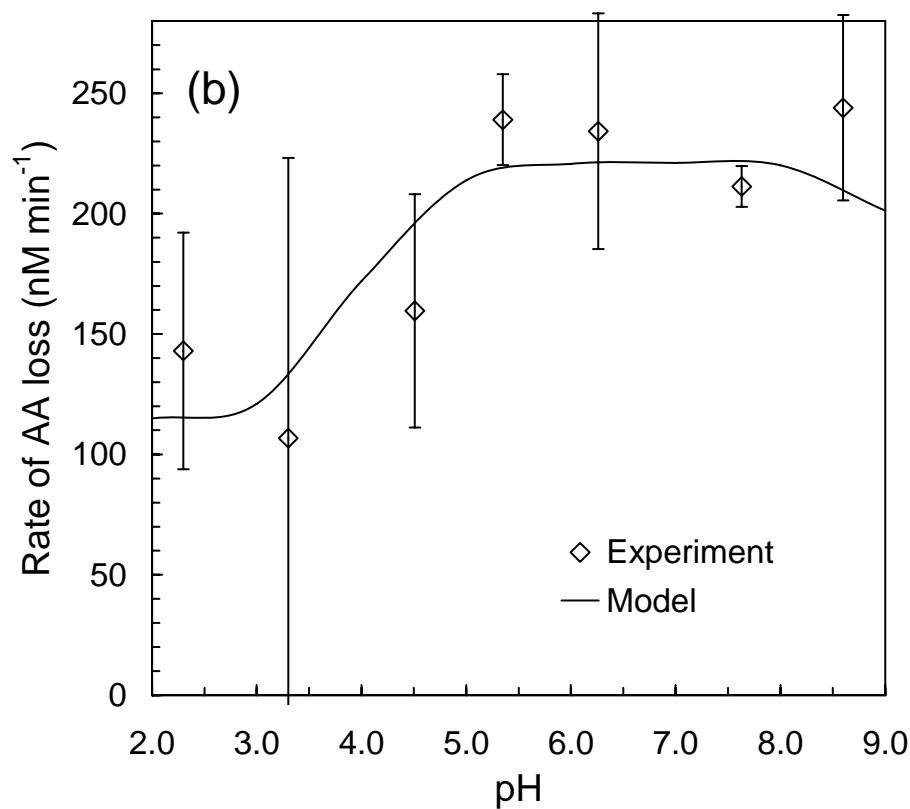
Fig. 4. (b) Rate of AA loss as a function of pH in the illuminated aqueous bromide solutions described in Fig. 4a. The symbols, line, and error bars are the same as in Fig. 3.
