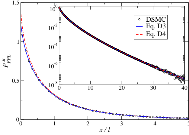
FIG. 12: (Color online) Free path length distribution for Maxwell molecules in two dimensions. The circles are the result of a DSMC simulation, while the solid line is the numerical integration of Eq. (D3). The dashed line is the large length approximation of Eq. (D4). All data are reported in units of mean free path.
