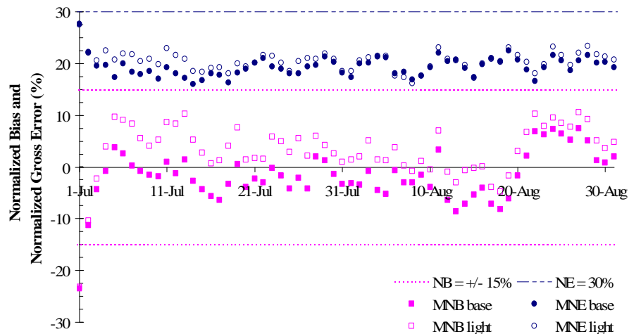
Fig. 1. Domain-wide daily normalized bias and error for O 3 in CMAQ when compared with AIRS, CASTNET and SEARCH O 3 measurements (for all pairs of O 3 >40 ppbv).
