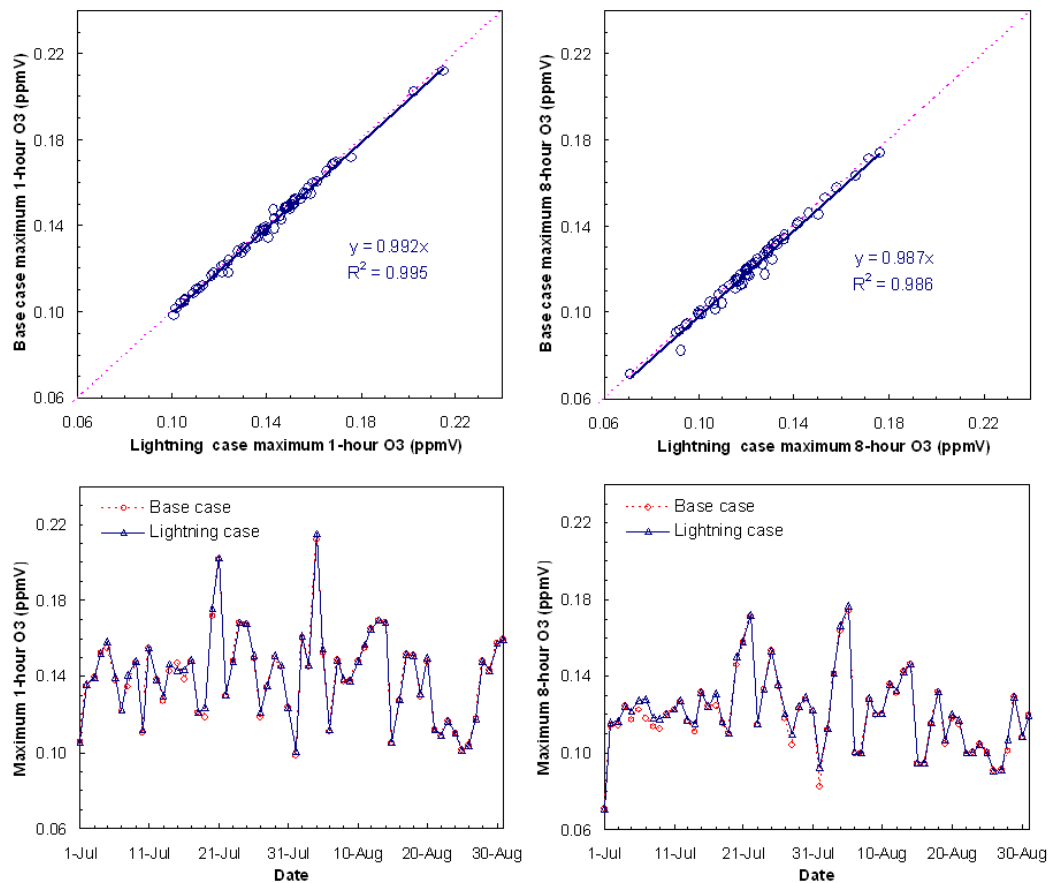
Fig. 5. Temporal evolution of domain-wide daily maximum 1-h (left panel) and 8-h (right panel) O 3 values with versus without lightning for July–August, 2004 (One grid with the maximum 1-h and 8-h O 3 is selected throughout the whole domain for each day).
