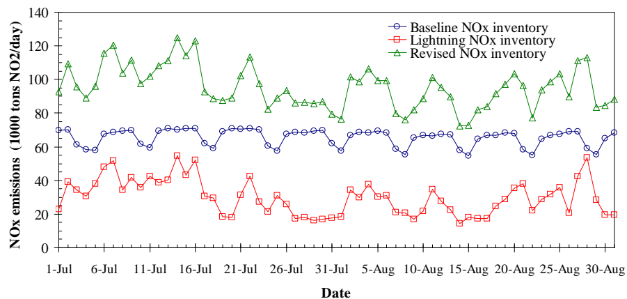
Fig. 3. Domain-wide baseline, lightning, and revised NO x emissions (as tons NO 2 /d) for July–August 2004.
