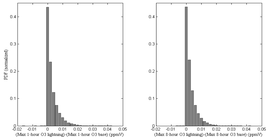
Fig. 6. Distribution of the change in daily 1-h and 8-h maximum O 3 values for model grids with AIRS ozone monitoring stations for July–August 2004.
