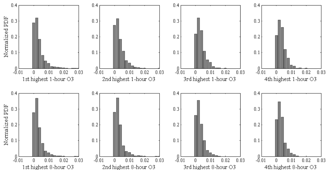
Fig. 9. Distribution of the difference (Lightning case-Base case) in the 1st, 2nd, 3rd and 4th highest 1-h (top) and 8-h (bottom) maximum O 3 values for grids with AIRS Ozone monitoring stations (PDF's are normalized and differences in units of ppmV).
