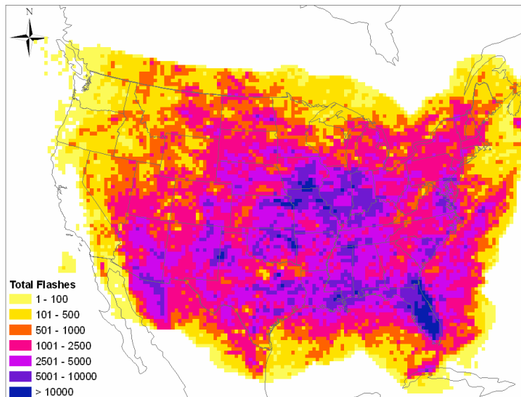
Fig. 4. Domain-wide lightning intensity map for July–August 2004.
