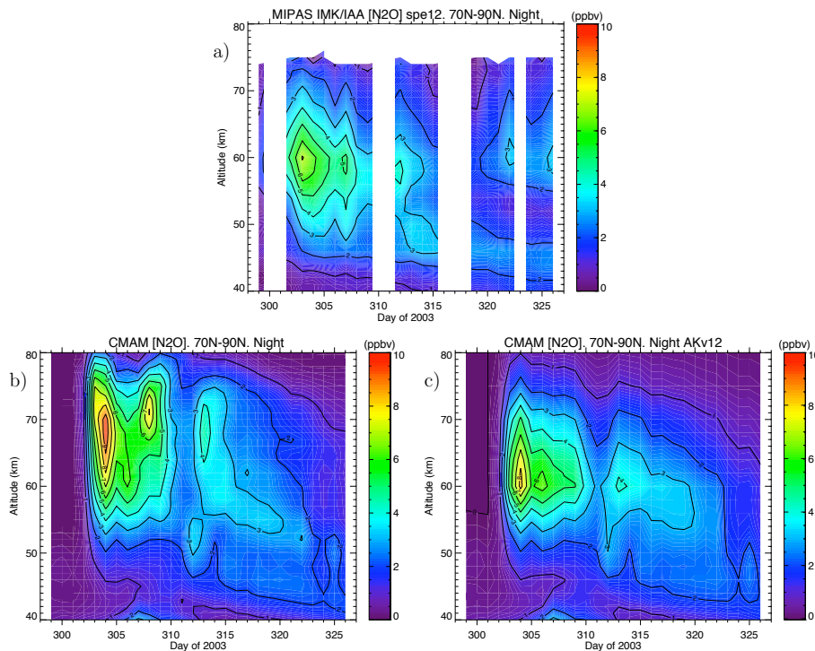
Fig. 5. Time series of N 2 O abundance after the solar proton events of October–November 2003 for the Northern Hemisphere polar cap (70–90° N) during nighttime conditions. (a) MIPAS measurements; where white areas at highest altitudes represent MIPAS measurements with no information and the vertical white bands represent days with no processed data. Lower panels: Simulations by the Canadian Middle Atmosphere Model without (b) and with (c) application of the averaging kernels of the MIPAS retrievals.
