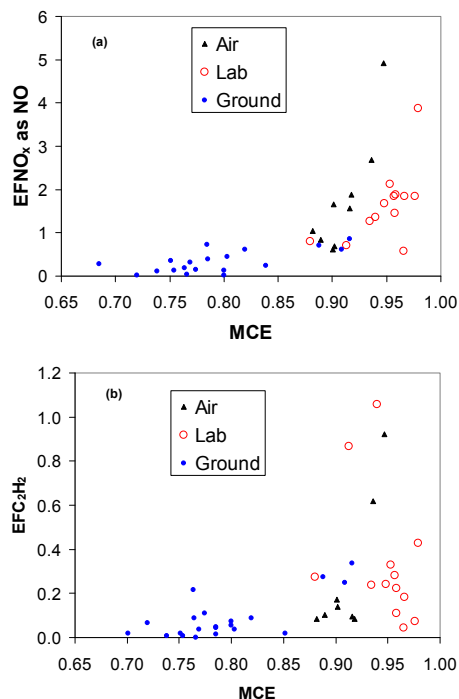
Fig. 3. Presentation of all the emission factors measured during TROFEE from ground-based, airborne, and laboratory platforms for NO x (a) and C 2 H 2 (b). Despite differences in fuels between the experiments, these compounds show a consistent trend of increasing emissions with increasing MCE indicating production mainly by weakly fuel-dependent flaming combustion. There is also a large range in the EF observed (factor of ~20).
