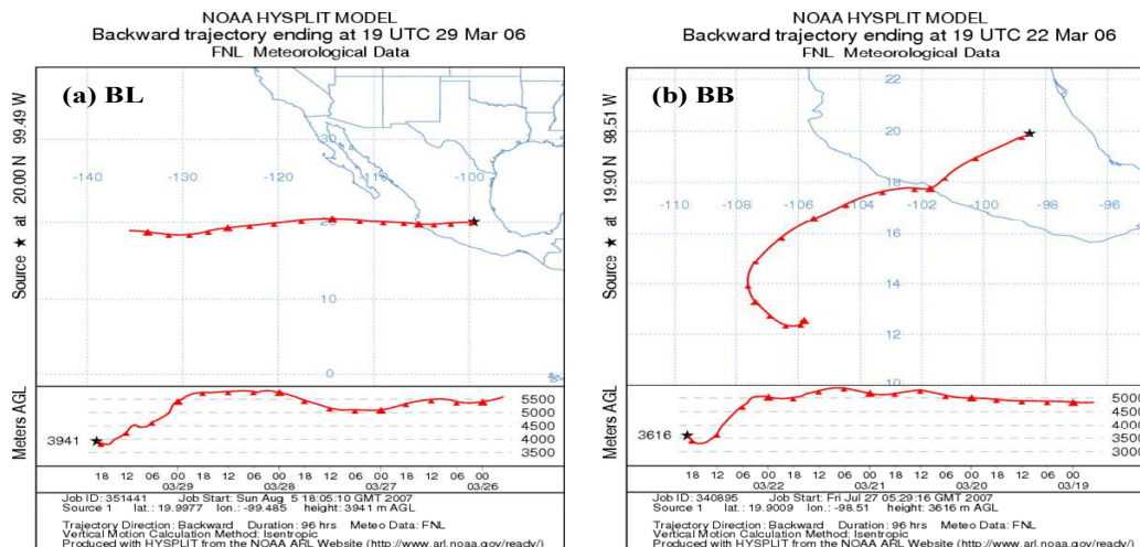
Fig. 4. Air mass back trajectory analysis for 5 air mass categories (BL (a) , BB (b) , FTCO (ac) , FTMA (d) , and TIC (e) ), which are the most frequent air mass back trajectory for each air mass category.
