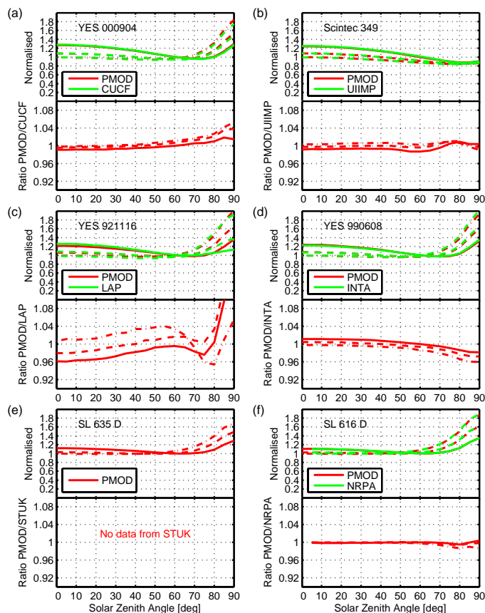
Fig. 3. Conversion function f in dependence of solar zenith angle for 200 DU (solid line), 300 DU (dashed line) and 400 DU (solid dashed line) calculated using the SRF measured, respectively, by PMOD/WRC and the home institute (see Fig. 1). The ratio of the two conversion functions are shown in the bottom half of each figure. The conversion function of the Solar Light 635 radiometer was not determined at STUK. 2272
