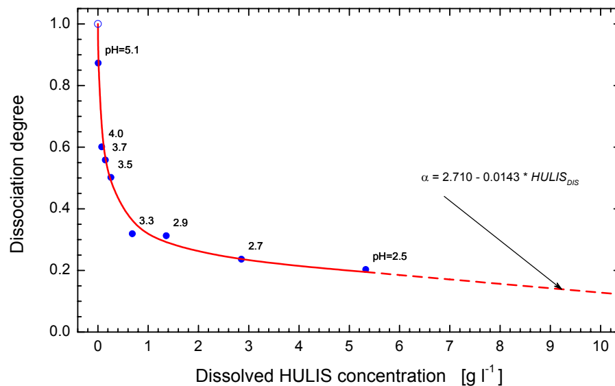
Fig. 4. Dissociation degree ( \alpha ) of pure HULIS solution with different dissolved HULIS concentration ( \text{HULIS}_{\text{DIS}} ). Solution pH values measured are also indicated. The connecting curve represents an eye-guide only.
