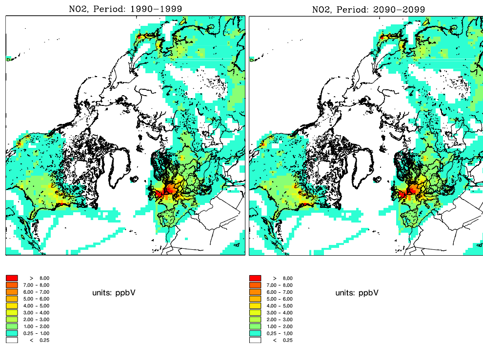
Fig. 11a and b. \text{NO}_2 , as in Fig. 7.
