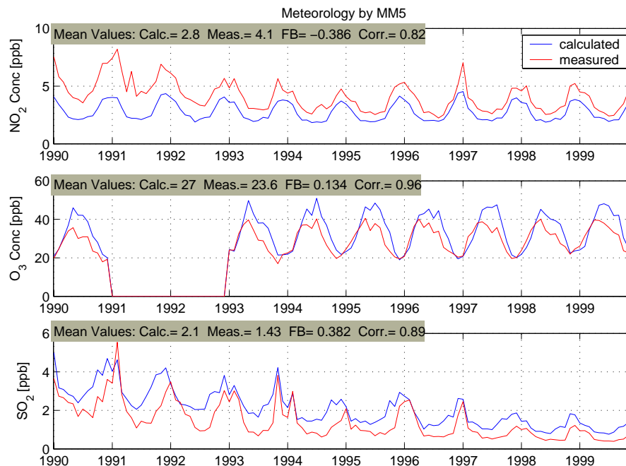
Fig. 2a. The calculated concentrations of \text{NO}_2 , \text{O}_3 , \text{SO}_2 and \text{SO}_4^{2-} as well as wet deposition of \text{SO}_4^{2-} and precipitation is compared with the observations from the EMEP measurement network (cf. Sect. 2.4) for the period 1990–1999. The data are monthly averaged values averaged over all the available measurement sites. The simulation is based on MM5 meteorology plus and 1990–1999 emissions. Also the mean values of the calculated and measured time series, the fractional bias (FB) and the correlation coefficient (Corr.) between the measured and calculated data series are displayed in each panel. For \text{O}_3 measurements are not available in 1991 and 1992.
