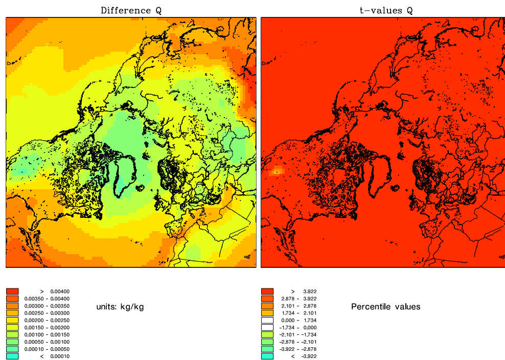
Fig. 6c and d. Continued.
