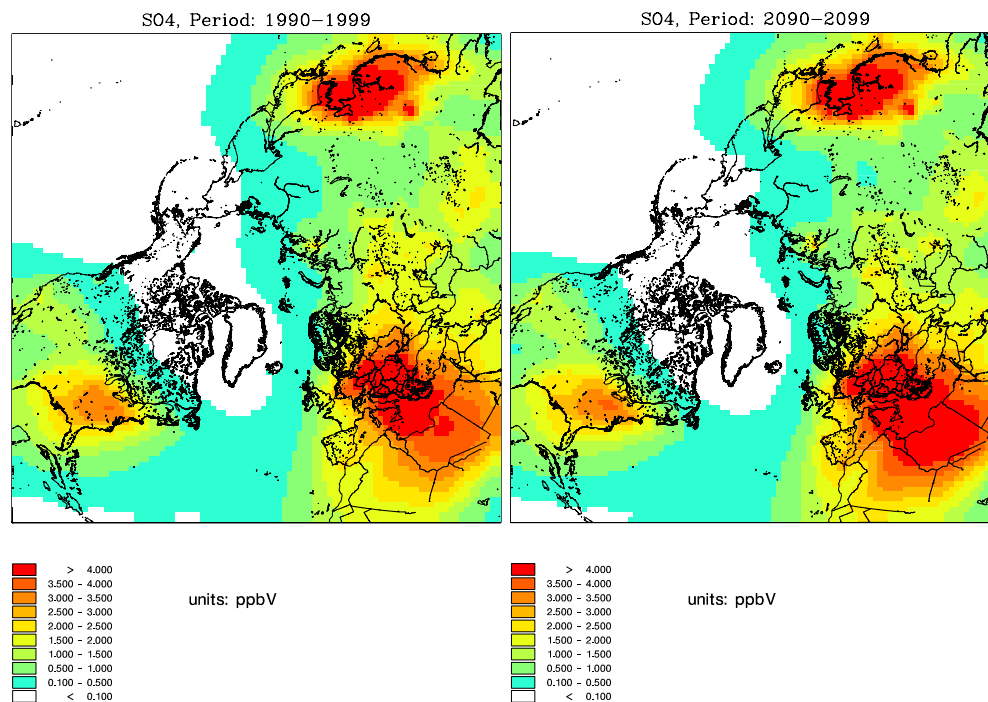
Fig. 8a and b. \text{SO}_4^{2-} concentration, as in Fig. 7.
