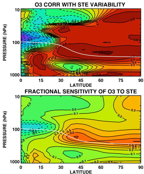
Fig. 8. Top panel: Distribution of linear correlation coefficients produced by regressing the monthly mean, zonal mean O_3 at each latitude and pressure level in the 4^\circ \times 5^\circ run of the Combo model with the monthly mean cross-tropopause flux of O_3 in the NH extratropics. Bottom panel: Fractional sensitivity of monthly mean, zonal mean O_3 in the 4^\circ \times 5^\circ run to changes in the cross-tropopause flux of O_3 in the NH extratropics. Fractional sensitivity is defined as the fractional change in O_3 mixing ratio per fractional change in the monthly mean cross-tropopause flux of O_3 , or S = m \times \langle F_{NH} \rangle / \langle O_3 \rangle , where m is the slope of the linear regression, \langle O_3 \rangle is the mean monthly mean, zonal mean O_3 over the 5-year model integration at some latitude and pressure, and \langle F_{NH} \rangle is the 5-year mean NH O_3 flux.
