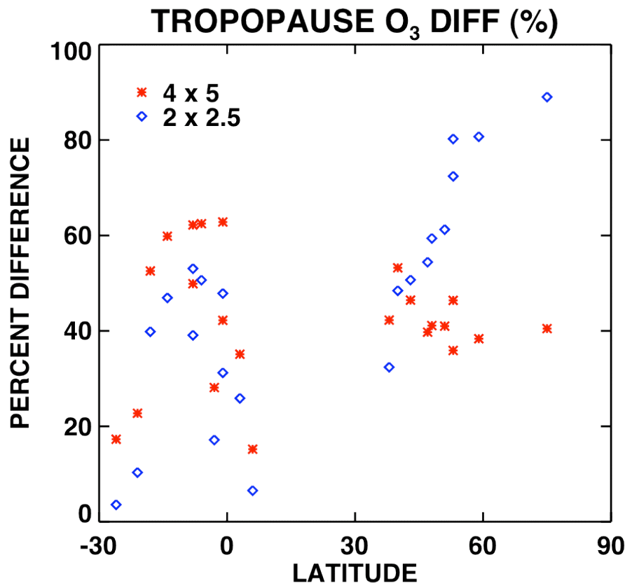
Fig. 7. Percent difference between modeled and observed annually averaged tropopause ozone for all stations, as a function of station latitude. Red asterisks show results from 4^{\circ} \times 5^{\circ} run, blue diamonds show results from 2^{\circ} \times 2.5^{\circ} run.
