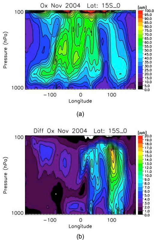
Fig. 10. (a) Zonal distribution of ozone from GEOS-Chem averaged in 15° bins in longitude and latitude from the equator to 15° S. (b) Average difference in GEOS-Chem ozone fields between a priori and a posteriori emissions based on 15° × 15° bins.
