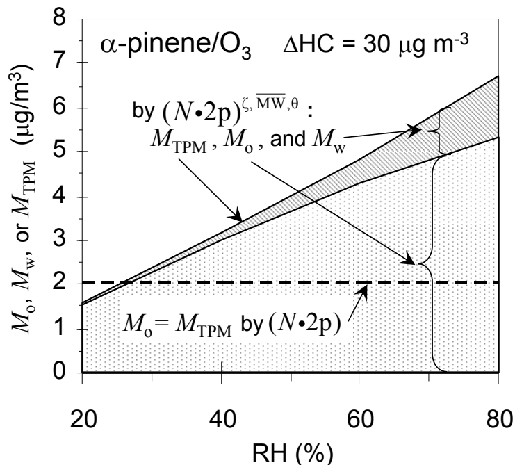
Fig. 6. M_o , M_w , and M_{\text{TPM}} by the (N \cdot 2p)^{\zeta, \overline{MW}, \theta} approach using the CP-Wilson.1 method for the activity coefficients for the \alpha -pinene/ \text{O}_3 products, with \Delta\text{HC} = 30 \mu\text{g m}^{-3} ; for comparison, M_o = M_{\text{TPM}} by the N \cdot 2p approach is also given.
