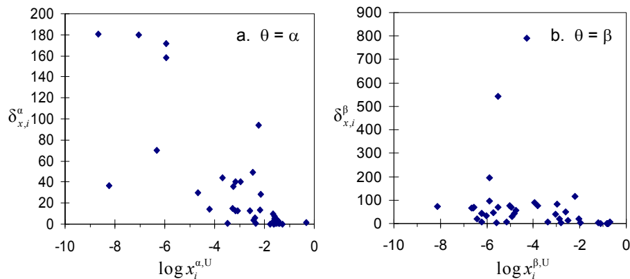
Fig. 3. Unsigned percentage difference between the values of x_i^\theta as predicted using CP-W.1 and UNIFAC plotted vs. \log x_i^{\theta,U} (U=UNIFAC) for \theta=\alpha and for \theta = \beta in the performance evaluation (PE) case.
