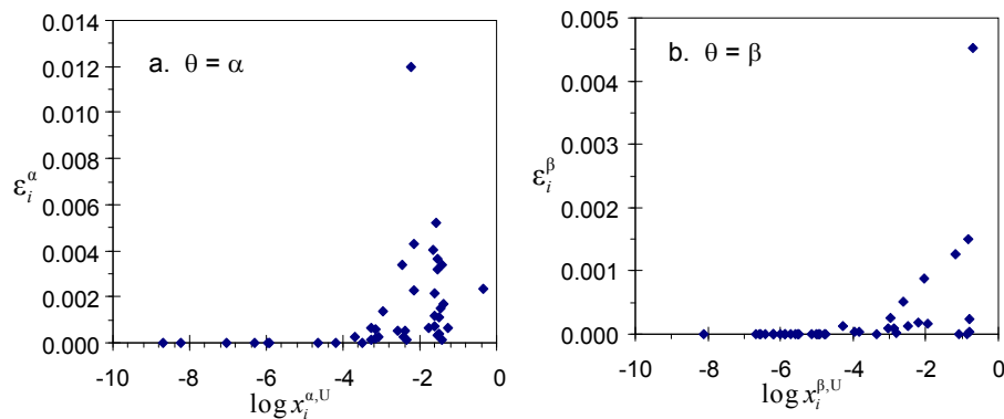
Fig. 4. Unsigned difference between the values of \mathcal{F}_i^\theta as predicted using CP-Wilson.1 and UNIFAC expressed as a percentage of (M_{\text{TPM}})^U vs. \log x_i^{\theta,U} ( U=\text{UNIFAC} ) for \theta=\alpha and for \theta=\beta in the performance evaluation (PE) case.
