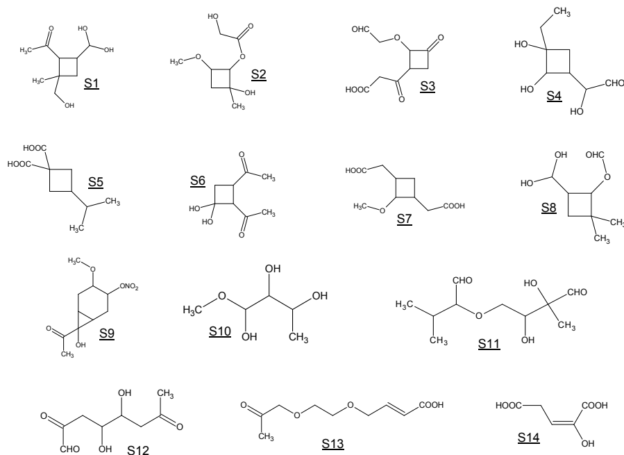
Fig. 1a. Molecular structures of lumped SOA products and surrogate POA compounds. \ddagger R 1 =C 15 alkyl chain; R 2 =C 17 alkyl chain; R 3 =C 17 alkyl chain with one double bond. For some structures, ether linkages have been included to fine tune the estimated polarity, even when such linkages may be unlikely consequences of the relevant oxidation reactions.
