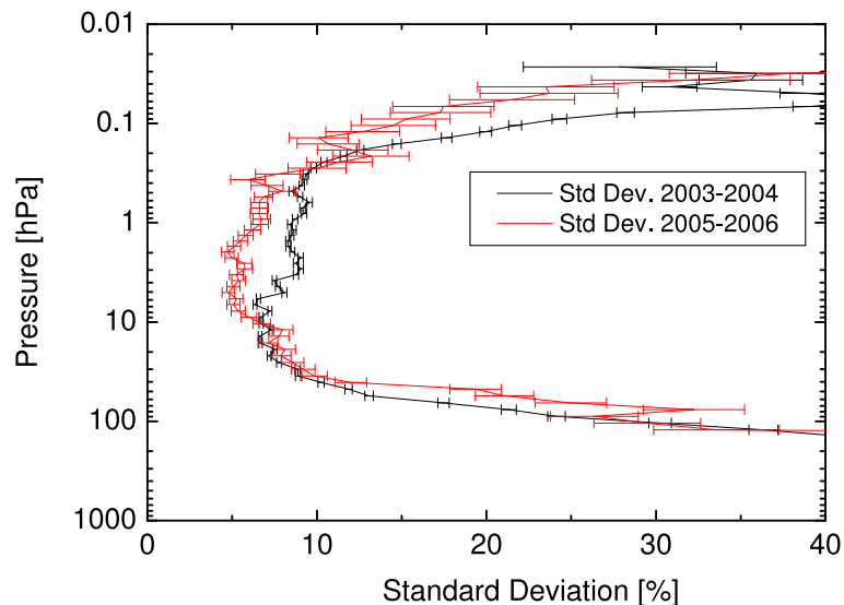
Fig. 6. Standard deviation of the differences between GOMOS and MIPAS ozone profiles as a percentage of the GOMOS mean profile, calculated for MIPAS full-resolution (2003–2004, in black) and reduced-resolution (2005–2006, in red) datasets.
