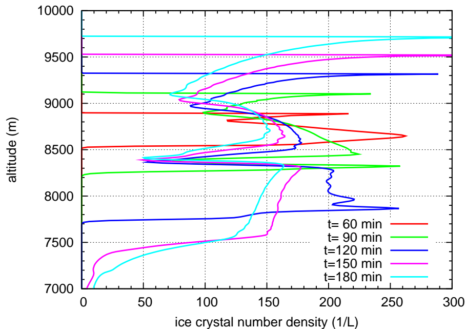
Fig. 21. Ice crystal number densities for w=0.08 \text{ m s}^{-1} at different simulation times. For the early simulation times, the moving peak is visible, while for t_s=90/120 \text{ min} , the in-cloud nucleation event in the vertical range 7700 \leq z \leq 8400 \text{ m} appears. The ice crystals, formed in the secondary nucleation event are then dispersed over the lower part of the cloud ( T_s=150/180 \text{ m} ). This leads to a layer structure of the cirrus cloud.
