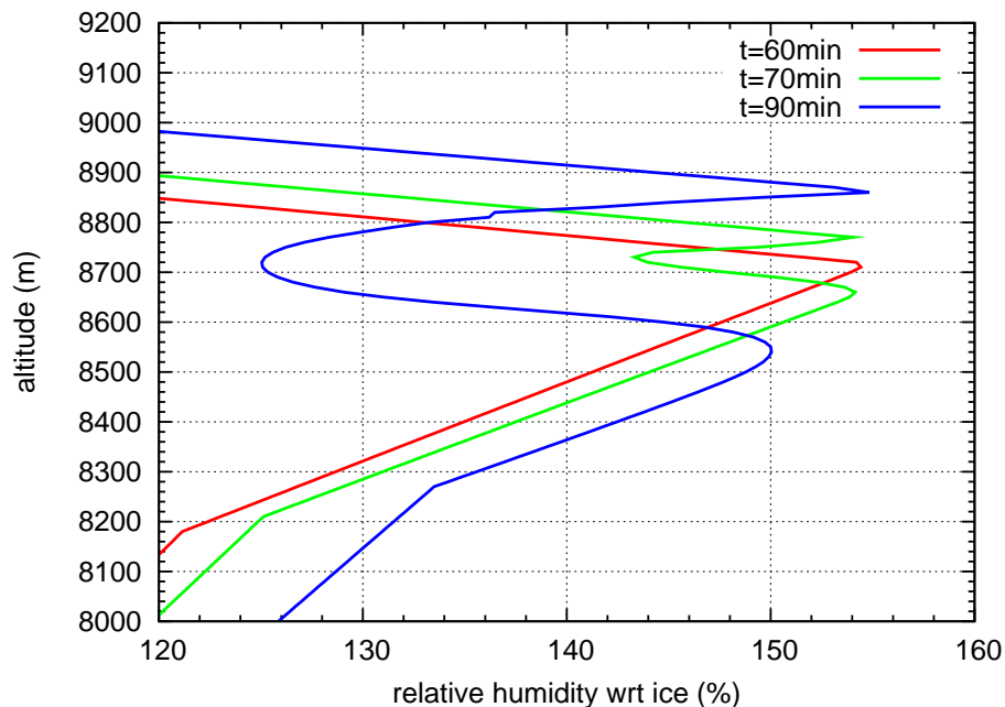
Fig. 16. Temporal evolution of the vertical RHi profiles for simulation time 60 \leq t \leq 90 min. The notch of the profile due to ice crystal growth is represented clearly, while the supersaturation at the cloud top remains.
