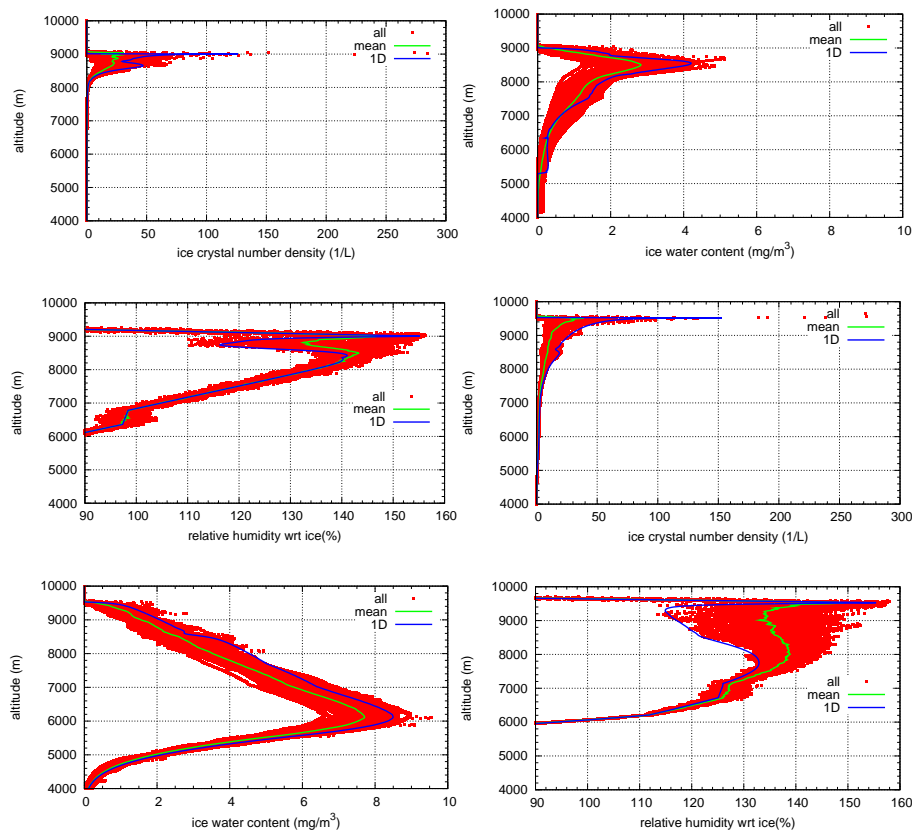
Fig. 23. Ice crystal number density (left), ice water content (middle) and relative humidity wrt ice (right) at t_s=120 min (top panel) and at t_s=240 min (bottom panel) for a constant updraught of w=0.05 m s -1 and additional temperature fluctuations. The values at all grid points are indicated by the red dots, the mean value is represented by the green line and the blue line indicates the values of the corresponding 1-D simulation.
