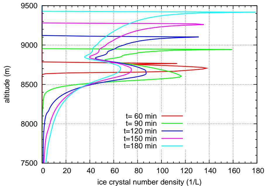
Fig. 18. Downward moving peak of ice crystal number density for the first nucleation event in the simulation with constant uplift of w=0.0\text{ m s}^{-1} . The peak is much more pronounced as in Fig. 17 due to higher ice crystal densities due to the stronger updraught.
