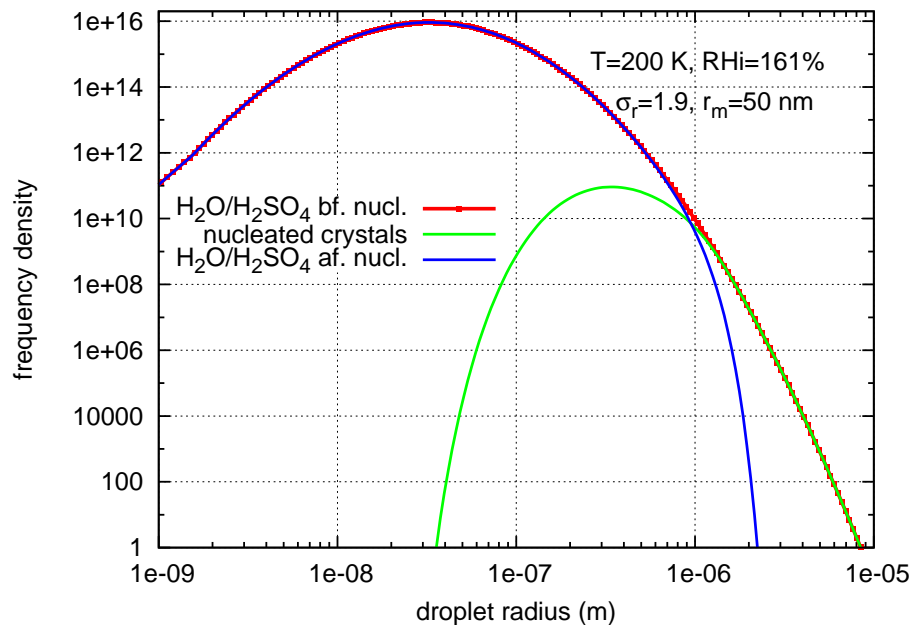
Fig. 8. Effect of a nucleation event during a time step of \Delta t=0.1\text{ s} at T=200\text{ K} and a relative humidity wrt ice RH_i=161\% for a quite broad aerosol distribution ( r_m=50\text{ nm} , \sigma_r=1.9 ): The \text{H}_2\text{O}/\text{H}_2\text{SO}_4 droplet distribution before the nucleation event is indicated by the red line points, the green line indicates the distribution of freshly nucleated ice crystals and the blue line describes the \text{H}_2\text{O}/\text{H}_2\text{SO}_4 droplet distribution after the nucleation event.
