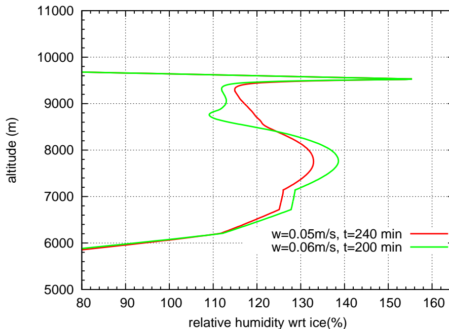
Fig. 19. Vertical RH i -profiles for the simulations at the same altitude, i.e. at equivalent times: t_s(w=0.05 \text{ m s}^{-1})=240 \text{ min} and t_s(w=0.06 \text{ m s}^{-1})=200 \text{ min} , respectively.
