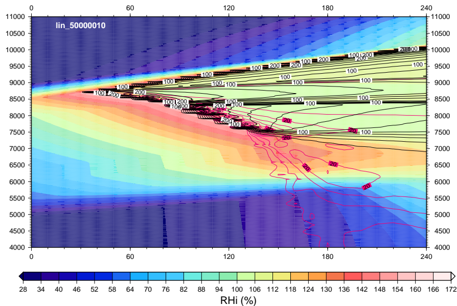
Fig. 20. Time evolution of the simulated cirrostratus lifted with a constant vertical velocity of w=0.08\text{ m s}^{-1} . The colours indicate relative humidity wrt ice, while lines indicate ice crystal number densities (black, in \text{L}^{-1} ) and ice water content (purple, in \text{mg m}^{-3} ).
