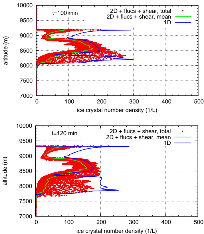
Fig. 26. Ice crystal number densities for a vertical updraught of w=0.08 \text{ m s}^{-1} with fluctuations and wind shear (red dots: all grid points, green line: mean value) and in the corresponding 1-D simulation (blue line) for t=100 \text{ min} (top) and 120 \text{ min} (bottom), respectively. In contrast to the simulations including only temperature fluctuations (Fig. 24), here the incloud nucleation events at the cloud bottom occur; however, they are weaker than in the pure 1-D simulations.
