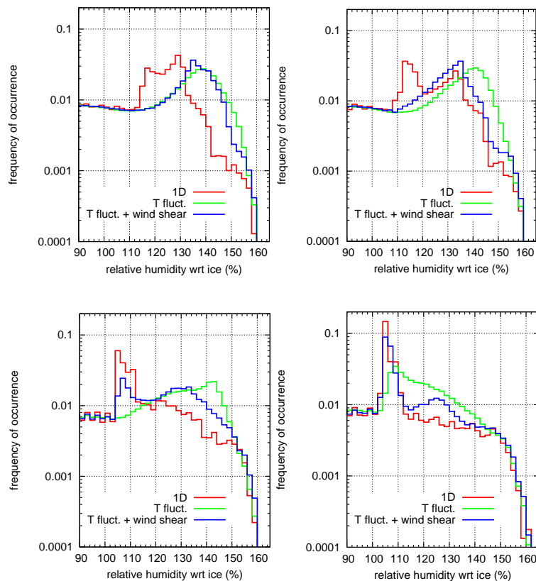
Fig. 27. Statistics of the relative humidity wrt ice for the simulations with different prescribed vertical velocities, from left to right: w=0.05 \text{ m s}^{-1} , w=0.06 \text{ m s}^{-1} , w=0.08 \text{ m s}^{-1} , w=0.1 \text{ m s}^{-1} , respectively. Here, all data from the whole simulation are collected, respectively. Red lines indicate the 1-D simulations, green lines denote 2-D simulations with temperature fluctuations and blue lines are 2-D simulations with temperature fluctuations and wind shear.
