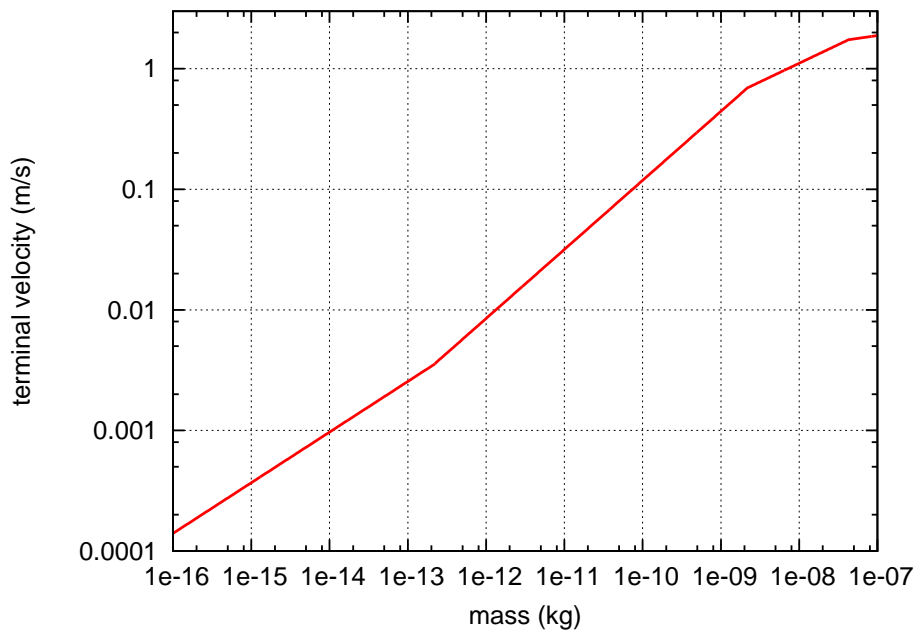
Fig. 3. Terminal velocity v(m) of a single ice crystal as function of the crystal mass m .
