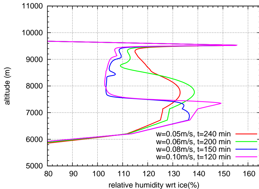
Fig. 22. Vertical RH i profile at the same altitude, i.e. at equivalent simulation times for all four simulations with different vertical updraught ( w=0.05/0.06/0.08/0.1\text{ m s}^{-1} ).
