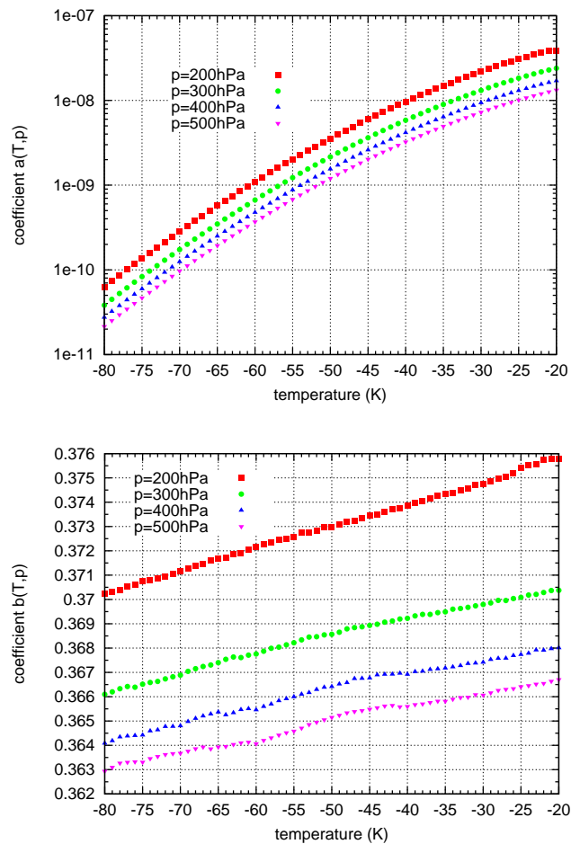
Fig. 4. Coefficients a(p, T) (top) and b(p, T) (bottom) for Koenig's ansatz dm/dt \approx a(p, T)m^{b(p, T)} and the approximation of the numerical solution of Eq. (30) for different pressures.
