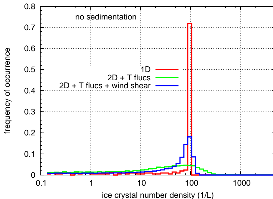
Fig. 28. Ice crystal number densities for three reference simulations (pure 1-D, temperature fluctuations, temperature fluctuations plus wind shear) without sedimentation. The whole model domain is lifted up with a constant vertical velocity of w=0.05 \text{ m s}^{-1} . Again, all data for the whole simulation are collected, respectively. The frequency of occurrence of the ice crystal number densities is indicated by the coloured lines (red: pure 1-D, green: temperature fluctuation, blue: temperature fluctuations plus wind shear). The impact of the horizontal and vertical small scale motions, triggered by the temperature fluctuations is clearly visible.
