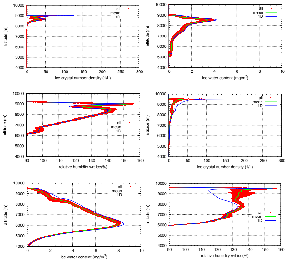
Fig. 25. Ice crystal number density (left), ice water content (middle) and relative humidity wrt ice (right) at t_s=120 min (top panel) and at t_s=240 min (bottom panel) for a constant updraught of w=0.05 m s -1 , additional temperature fluctuations and wind shear. The values at all grid points are indicated by the red dots, the mean value is represented by the green line and the blue line indicates the values of the corresponding 1-D simulation.
