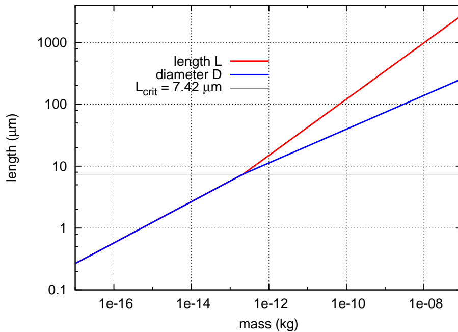
Fig. 1. Length ( L ) and diameter ( D ) of hexagonal ice crystals as functions of the ice crystal mass m .
