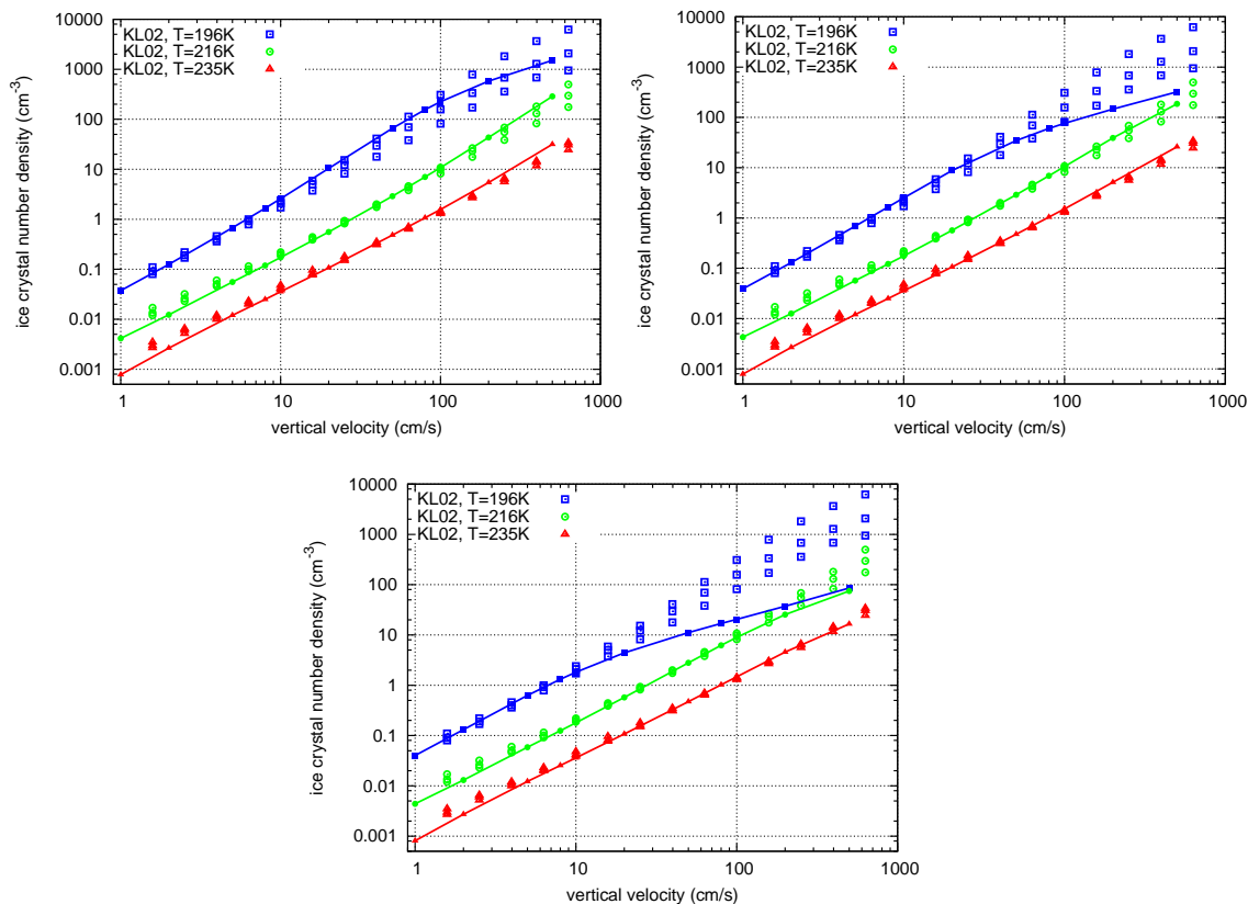
Fig. 7. Box model calculations for the homogeneously formed ice crystal number densities depending on the vertical velocity. The calculations for different temperatures are indicated by the colours (red: T=235\text{ K} , green: T=216\text{ K} , blue: T=196\text{ K} ). Line points indicate calculations with our box model, points denotes values from Kärcher and Lohmann (2002a) . The panels show the impact of the width of the aerosol distribution: top: \sigma_r=1.3 , middle: \sigma_r=1.6 , bottom: \sigma_r=1.9 .
