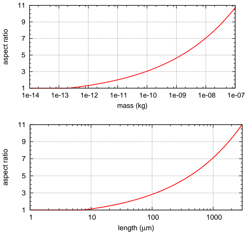
Fig. 2. Aspect ratio r_a of hexagonal ice crystals versus ice crystal mass m (upper panel) and length L (lower panel), respectively.
