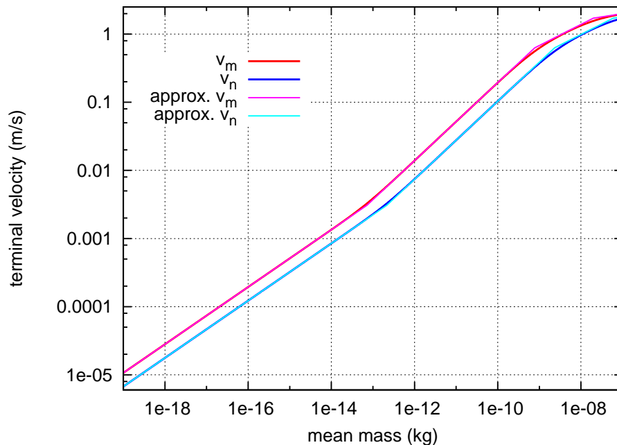
Fig. 6. Mean terminal velocities v_m , v_n for r_0=3 and the approximations by using the expressions of general moments as in Eq. (50) as piecewise functions.
