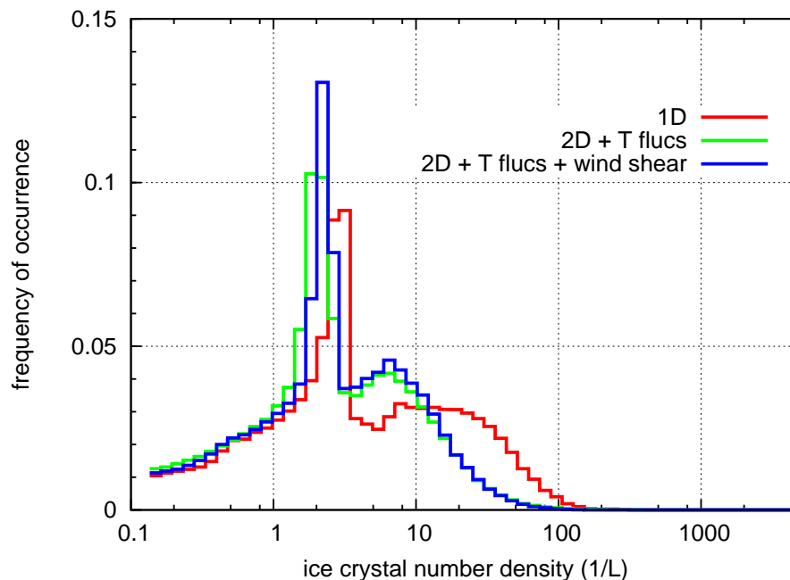
Fig. 29. Ice crystal number densities for three reference simulations (pure 1-D, temperature fluctuations, temperature fluctuations plus wind shear) with sedimentation. The whole model domain is lifted up with a constant vertical velocity of w=0.05 \text{ m s}^{-1} . Again, all data for the whole simulation are collected, respectively. The frequency of occurrence of the ice crystal number densities is indicated by the coloured lines (red: pure 1-D, green: temperature fluctuation, blue: temperature fluctuations plus wind shear). In comparison with Fig. 28, sedimentation influences already the pure 1-D case dispersing the ice crystal number density over the whole cloud which leads to a shift in the frequency of occurrence towards smaller densities.
