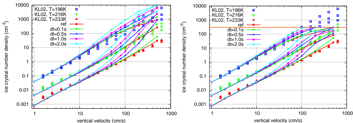
Fig. 13. Box model calculations for the homogeneously formed ice crystal number densities depending on the vertical velocity and on the temperature. For comparison, the values from detailed microphysics calculations in Kärcher and Lohmann (2002a) are shown. For the simulations, we assume a fixed width for the aerosol distribution of \sigma_r=1.4 and a geometric mean radius of r_m=25 nm. Here, the impact of the prescribed (fixed) time step ( dt=0.1/0.5/1.0/2.0 ) for the simulations is shown, compared to simulations using an adapted time step (simulation “ref”, red line). For the simulations shown at the top panel, the background aerosol reservoir is large, while for the simulations at the bottom panel, we used a realistic background aerosol concentration ( n_c=300 cm -3 ).
