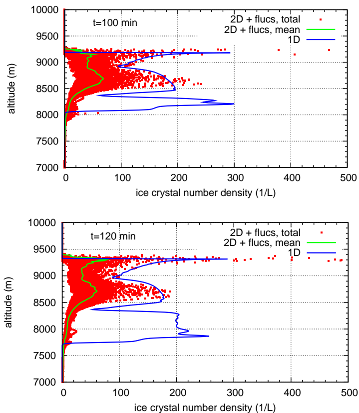
Fig. 24. Ice crystal number densities for a vertical updraught of w=0.08 \text{ m s}^{-1} with fluctuations (red dots: all grid points, green line: mean value) and in the corresponding 1-D simulation (blue line) for t=100 \text{ min} (top) and 120 \text{ min} (bottom), respectively. In the simulation including fluctuations the inside cloud nucleation events are missing at the bottom of the cloud, compared to the 1-D case.
