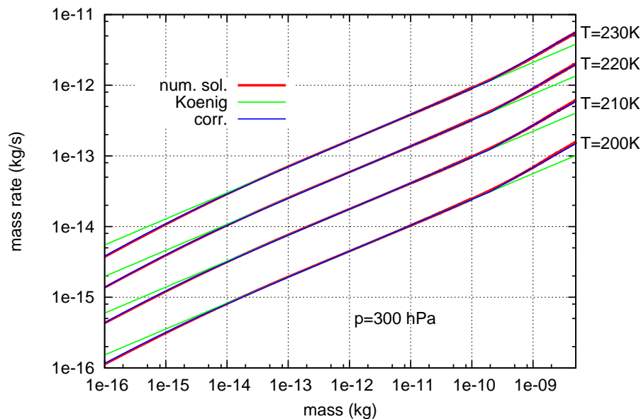
Fig. 5. Approximation of single ice crystal growth rates dm/dt (red) using the original Koenig ansatz (green) and the Koenig ansatz with our corrections (blue) for different temperatures ( T=230/220/210/200 K) and fixed pressure ( \rho=300 hPa).
