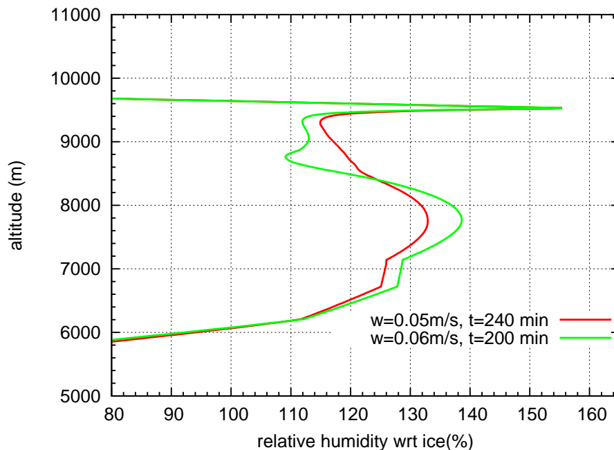
Fig. 19. Vertical RH i -profiles for the simulations at the same altitude, i.e. at equivalent times: t_s(w=0.05\text{ m s}^{-1})=240\text{ min} and t_s(w=0.06\text{ m s}^{-1})=200\text{ min} , respectively.
