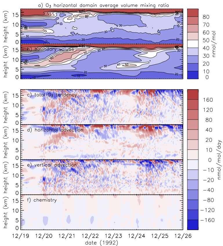
Fig. 13. As Fig. 11 for the LTN1 run.
