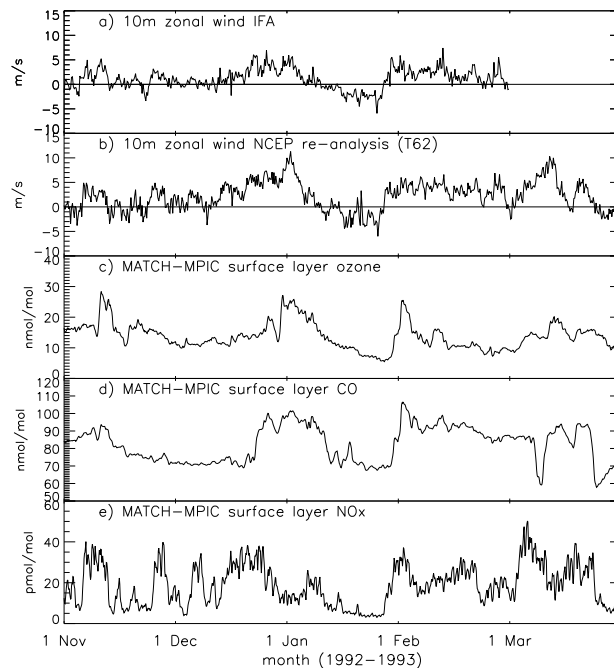
Fig. 18. Time series of (a) 10 m observed zonal wind, (b) 10 m zonal wind from the interpolated NCEP re-analysis data (see Sect. S8), (c) O 3 volume mixing ratio in the lowest model layer (surface layer) calculated by MATCH-MPIC, (d) surface layer CO, (e) surface layer NO x at the site of the TOGA COARE IFA.
