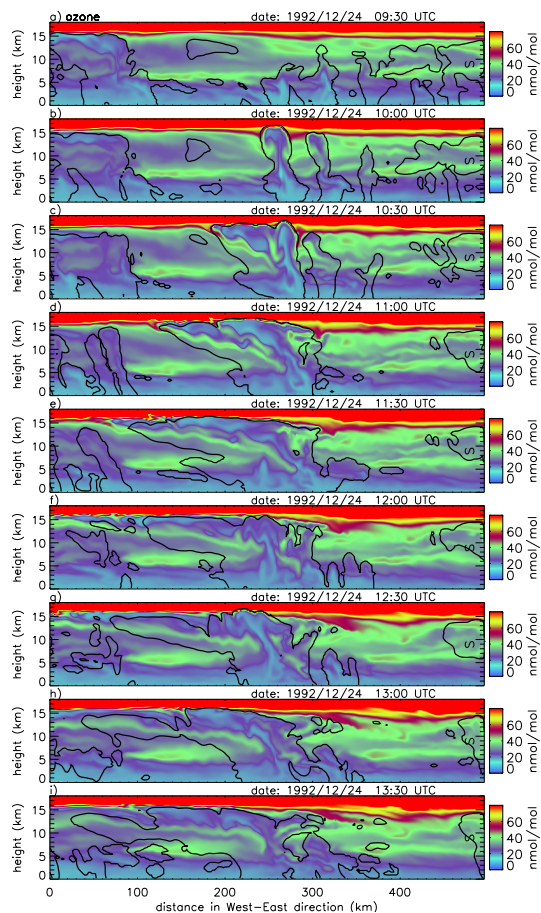
Fig. 16. \text{O}_3 volume mixing ratios (filled) from the LTN1 run for 24 December 1992, 09:30 UTC to 13:30 UTC and total hydrometeor mixing ratio q_{\text{totm}} = 0.01 \text{ g kg}^{-1} contour.
