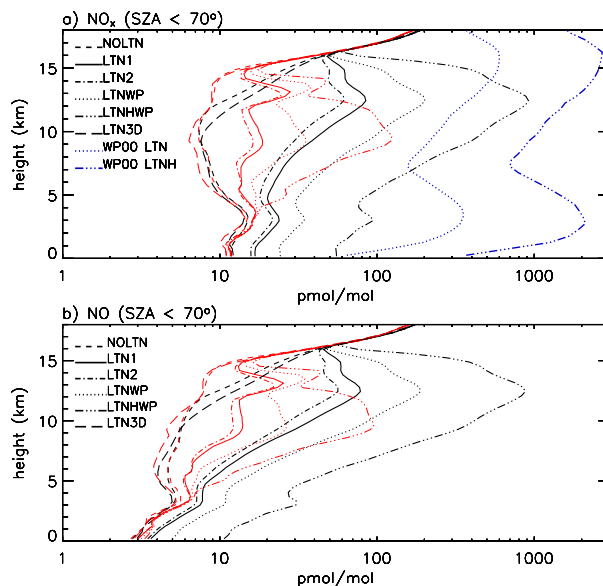
Fig. 5. Domain- and time-average (black lines) and median (red lines) volume mixing ratios of (a) NO x and (b) NO for solar zenith angles (SA) lower than 70°. Blue lines in (a): domain-averaged NO x volume mixing ratio from Fig. 11 of Wang and Prinn (2000) at the end of their LTN and LTNH runs.
