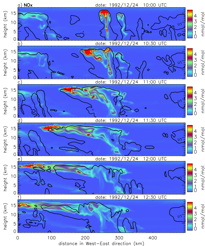
Fig. 7. NO x volume mixing ratios and the q_{\text{totm}} = 0.01 \text{ g kg}^{-1} contour (where q_{\text{totm}} = q_{\text{cloud water}} + q_{\text{rain}} + q_{\text{ice}} + q_{\text{graupel}} + q_{\text{snow}} is the sum of all hydrometeor mass mixing ratios) during the development of a mesoscale convective system from 24 December 1992, 10:00 UTC to 24 December 1992, 12:30 UTC from the LTN1 run. The time increment between the plots in each of the panels is 30 min.
