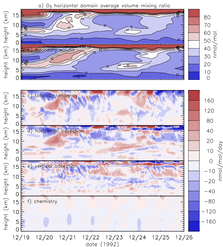
Fig. 11. (a) Time series of domain-averaged O 3 volume mixing ratios for the LTN3D run; (b) boundary values; (c)–(f) budget terms as defined by Eq. (2).
