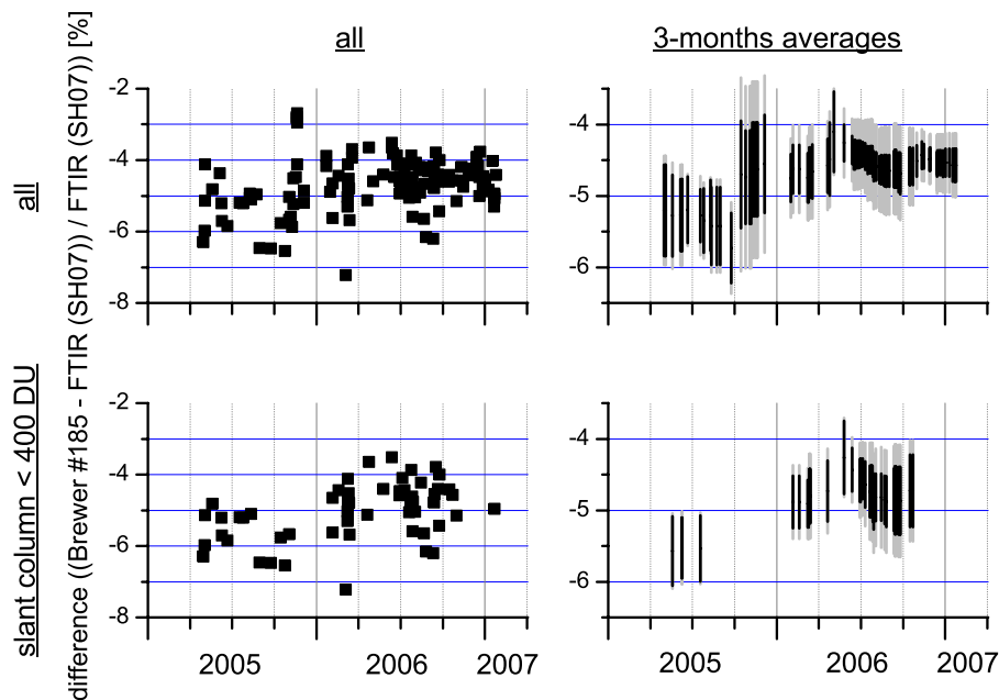
Fig. 10. Time series for the differences of total O_3 measured by the Brewer #185 and the FTIR. ( (\#185 - FTIR) / FTIR ). Content of panels, symbols, and colours is the same as in Fig. 3.
