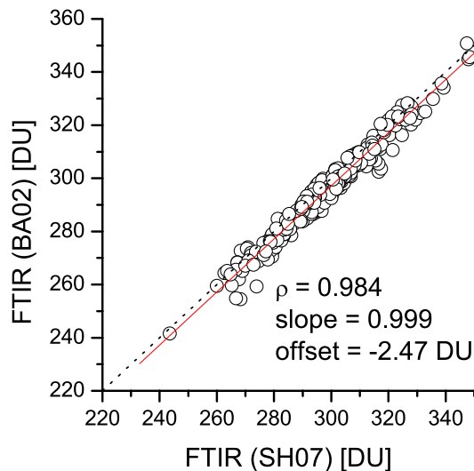
Fig. 5. Correlation between total column amounts for different FTIR approaches (a first similar to Barret et al. (2002) and a second according to Schneider and Hase (2007)). Black circles are individual measurements, red line linear regression lines of least squares fit.
