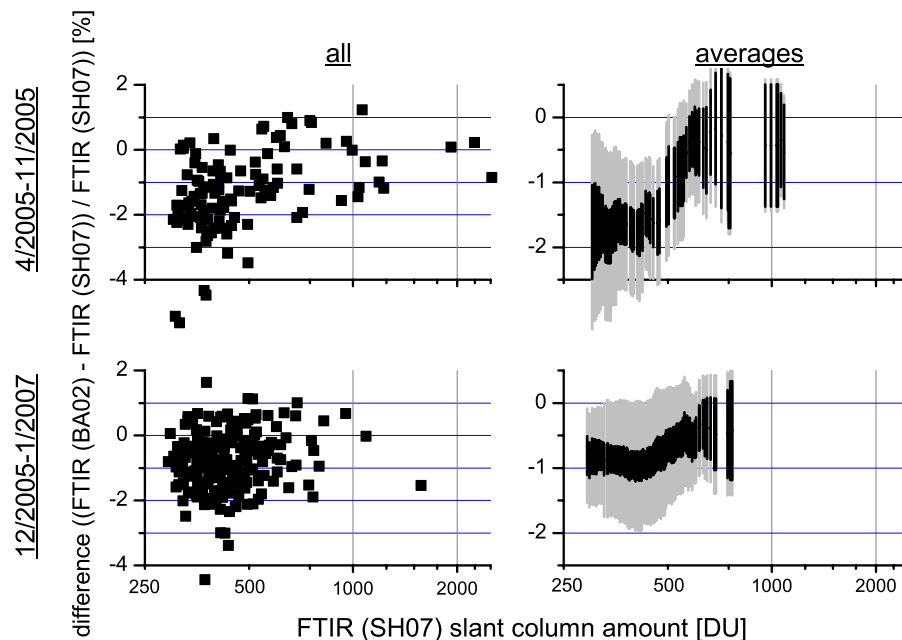
Fig. 7. Differences of total O_3 measured by the different FTIR approaches (FTIR (BA02)–FTIR (SH07)) / FTIR (SH07)) versus slant column amounts. Content of panels, symbols, and colours is the same as in Fig. 4.
