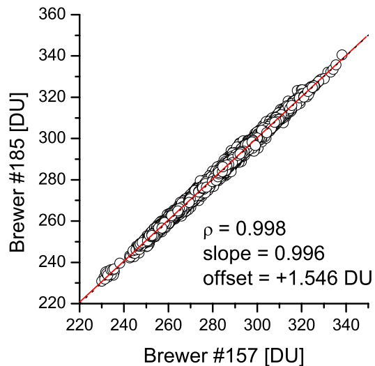
Fig. 2. Correlation between total column amounts of Brewer #157 and Brewer #185. Black circles are individual measurements, red line represents linear regression line of least squares fit.
