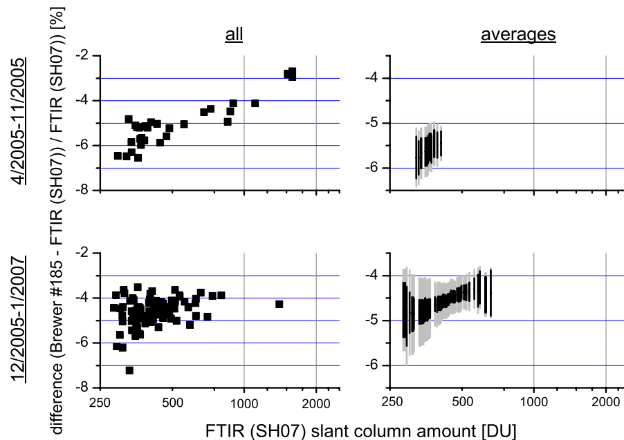
Fig. 12. Differences of total O_3 measured by the Brewer #185 and the FTIR. ((\#185 - \text{FTIR}) / \text{FTIR}) versus slant column amounts. Content of panels, symbols, and colours is the same as in Fig. 4.
