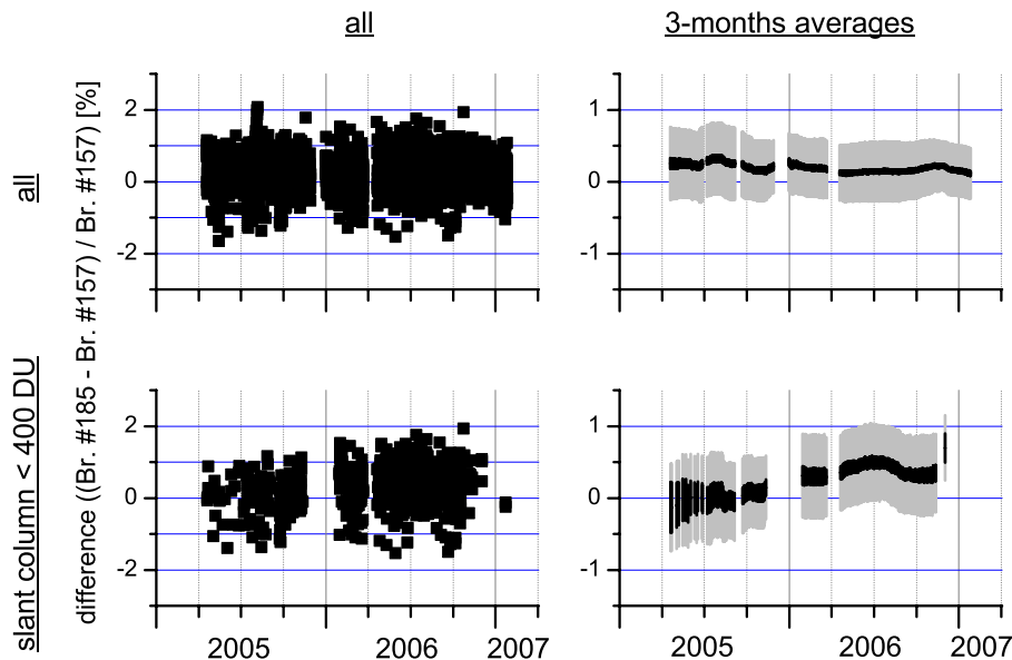
Fig. 3. Time series for the differences of total O_3 measured by the Brewer #157 and the Brewer #185 ( (\#185 - \#157) / \#157 ). Upper panels: for all coinciding measurements; bottom panels: for measurements with low slant columns ( <400 DU). The left panels show all individual coincidences and the right panels the statistics of three months averages: the black shaded area covers the range within which the mean value is situated with a probability of 95%; the grey-shaded area indicates the standard deviation. The scale of the y-axis of the right panels is extended by a factor 2.
