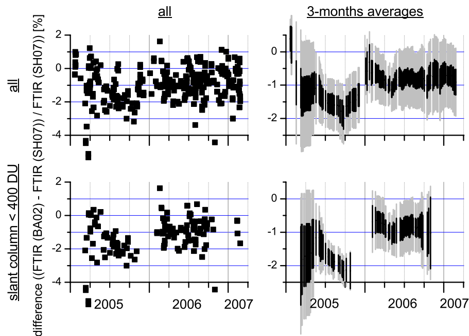
Fig. 6. Time series for the differences between the different FTIR approaches (FTIR (BA02)–FTIR (SH07)) / FTIR (SH07)). Content of panels, symbols, and colours is the same as in Fig. 3.
