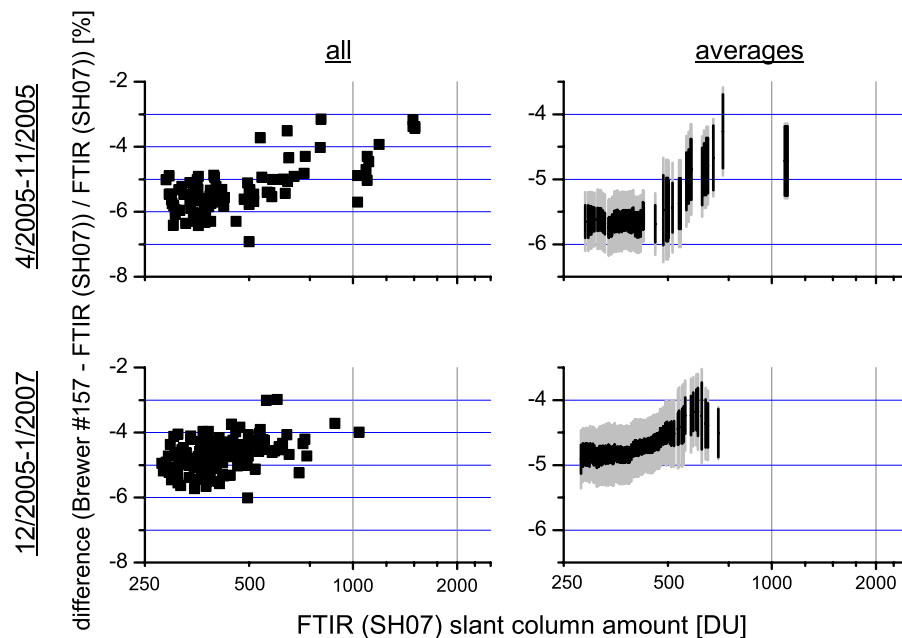
Fig. 11. Differences of total O_3 measured by the Brewer #157 and the FTIR. ((\#157 - \text{FTIR}) / \text{FTIR}) versus slant column amounts. Content of panels, symbols, and colours is the same as in Fig. 4.
