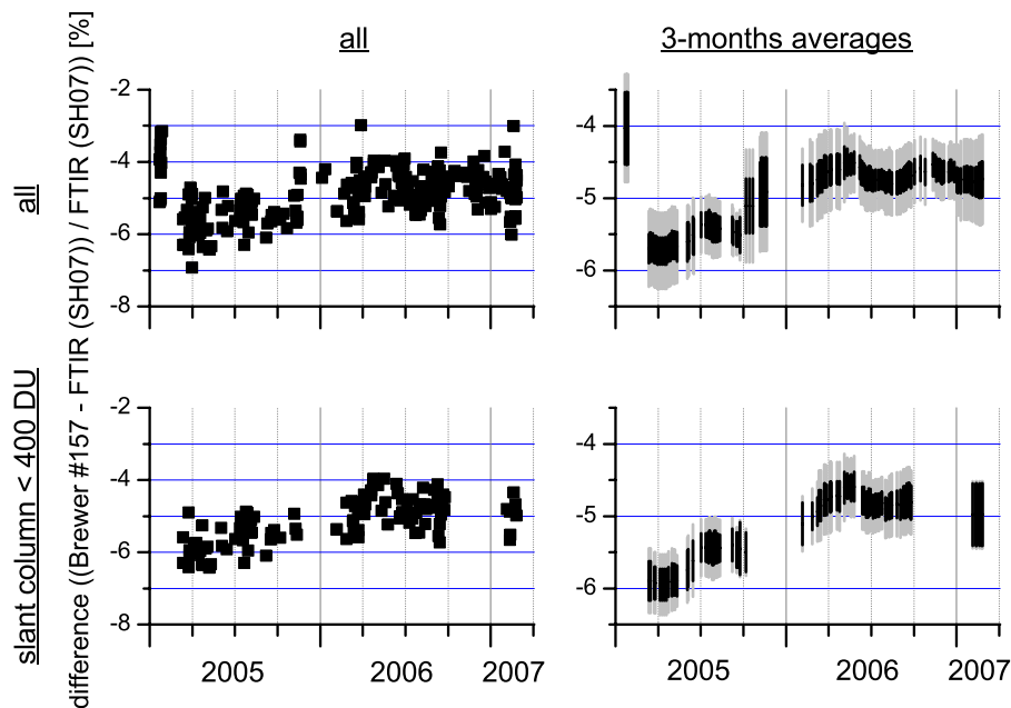
Fig. 9. Time series for the differences of total O 3 measured by the Brewer #157 and the FTIR. ((#157–FTIR) / FTIR). Content of panels, symbols, and colours is the same as in Fig. 3.
