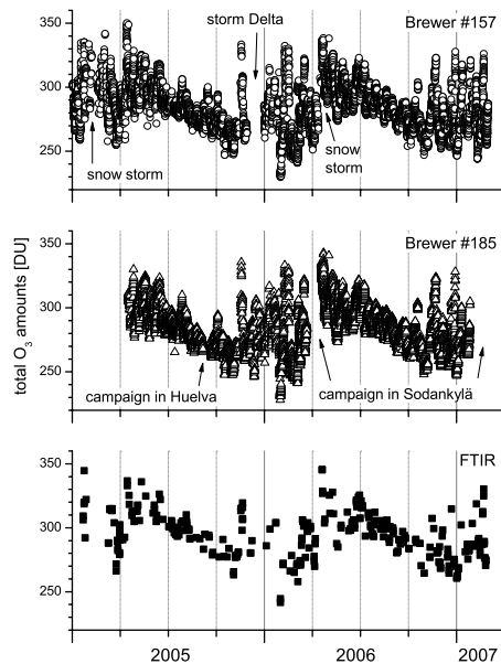
Fig. 1. Time series of total O 3 as measured by the Brewer site standard Brewer #157, the traveling standard Brewer #185, and the FTIR instrument.
