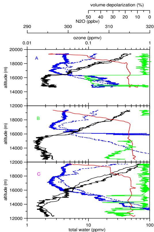
Fig. 10. Solid blue lines show the total water mixing ratio from FISH. Dashed blue lines show the water vapor saturation mixing ratio from temperature measurements. Black lines are ozone mixing ratios from FOZAN (the more structured one) and ECOC (the smoother one). Red lines are \text{N}_2\text{O} mixing ratio from HAGAR. Green lines show depolarization ratio from MAS. Data from MAS are missing for part of the flight. Upper, middle and lower panel are for profiles A, B and C respectively, as depicted in Fig. 2.
