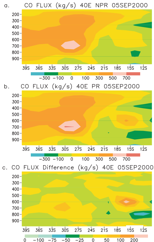
Fig. 12. Vertical cross sections of eastward CO flux ( \text{kg s}^{-1} ) over each latitude-altitude grid along the blue reference lines in Fig. 11 for the NPR run (a) , PR run (b) , and the corresponding difference between the PR and NPR runs (c) .
