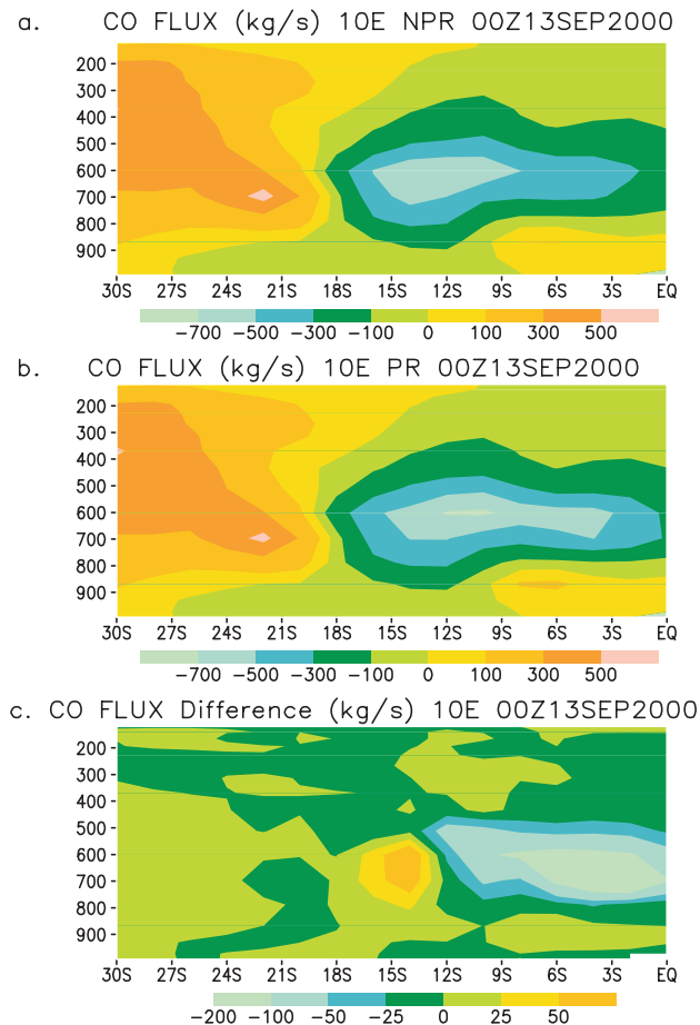
Fig. 10. Vertical cross sections of eastward CO flux ( \text{kg s}^{-1} ) over each latitude-altitude grid along the blue reference lines in Fig. 8 for the NPR run (a), PR run (b), and the corresponding difference between the PR and NPR runs (c).
