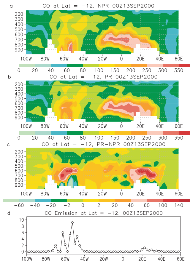
Fig. 9. Vertical cross sections of CO (ppb) along the red reference lines in Fig. 8 for the NPR run (a), PR run (b), and the concentration difference between PR and NPR runs (c). (d) Corresponding CO emission rate (kg s -1 ). White areas indicate topography.
