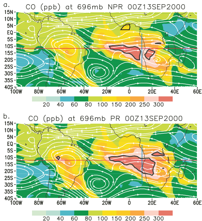
Fig. 8. Simulated CO concentrations for (a) the NPR run and (b) the PR run at 696 hPa in 13 September 2000. 3-day (10–12 September 2000) averaged streamlines in white are superimposed. The red and blue reference lines, used in Figs. 9 and 10, are drawn. Thick black line is the 300 ppb contour.
