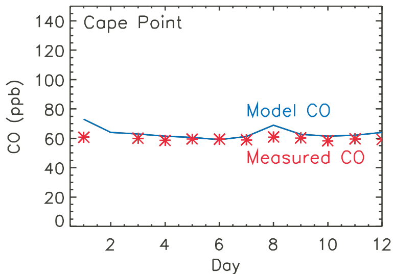
Fig. 4. Daily surface concentrations (ppb) of measured (red) and modeled CO (blue) over Cape Point, South Africa (34.4° S, 18.5° E) from 1 September 2000 to 12 September 2000.
