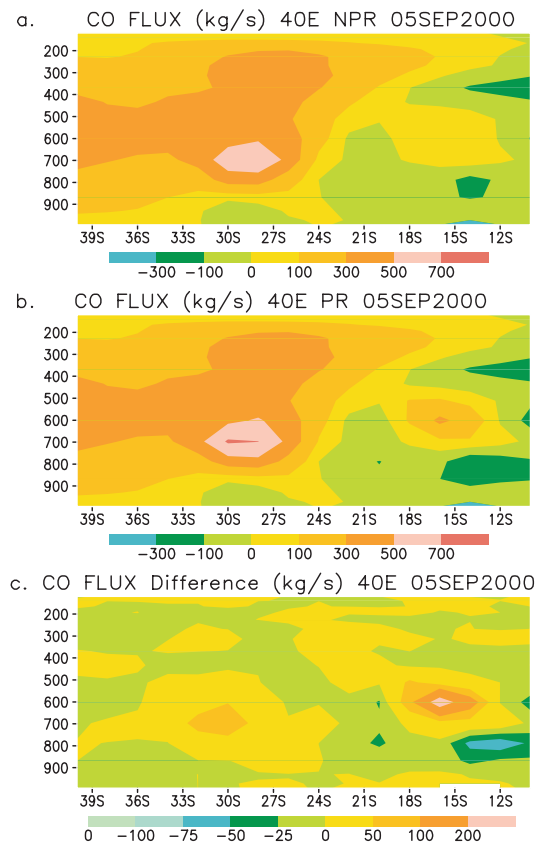
Fig. 12. Vertical cross sections of eastward CO flux ( \text{kg s}^{-1} ) over each latitude-altitude grid along the blue reference lines in Fig. 11 for the NPR run (a), PR run (b), and the corresponding difference between the PR and NPR runs (c).
