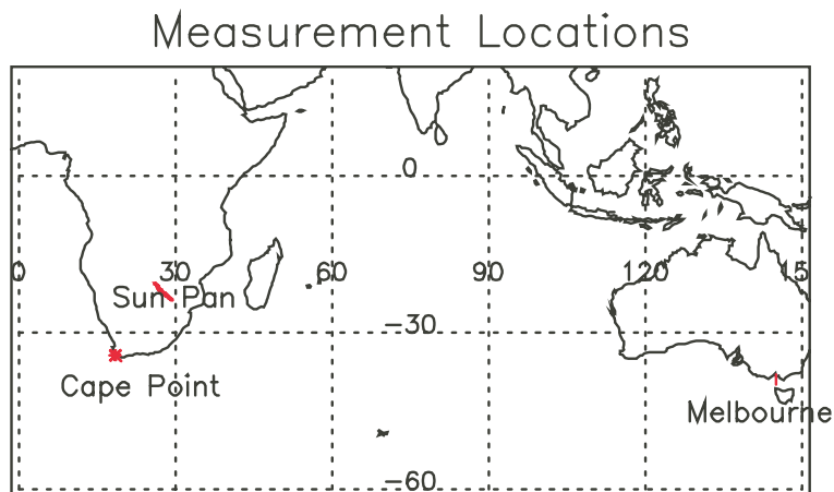
Fig. 1. Ground-based station (red star) and aircraft flight tracks for CO measurements (red lines).
