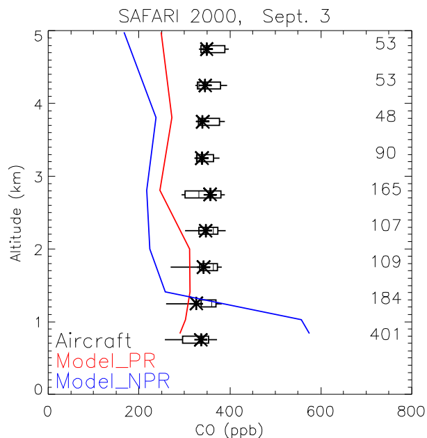
Fig. 6. CO vertical profiles averaged over 20–24° S and 24–30° E for 3 September 2000 from the model (red and blue lines) and South African aircraft measurement (black stars). The 25, 50, and 75 percentiles of the measured CO (ppb) are denoted by the vertical bars. The horizontal lines indicate the measurement ranges. The aircraft measurements are averaged over 500-m height range. The observation numbers in each height range are indicated.
