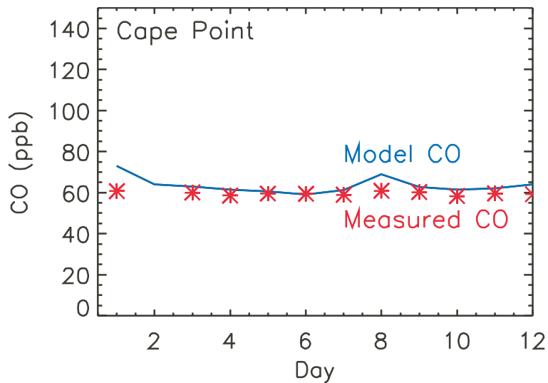
Fig. 4. Daily surface concentrations (ppb) of measured (red) and modeled CO (blue) over Cape Point, South Africa ( 34.4^{\circ} S, 18.5^{\circ} E) from 1 September 2000 to 12 September 2000.
