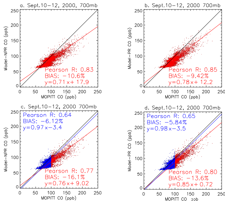
Fig. 3. Scatter plots of modeled versus MOPITT CO at 700 hPa in 10–12 September 2000 within the Fig. 2 domain for the NPR (a and c) and PR (b and d) runs. The black lines represent a 1:1 correlation. The red lines for a and b are the linear regression for CO data. The red and blue lines for c and d represent the linear regression for higher ( \geq 100 ppb) and lower ( < 100 ppb) MOPITT CO data, respectively. The Pearson correlation coefficients R, mean biases, and regression equations are indicated.
