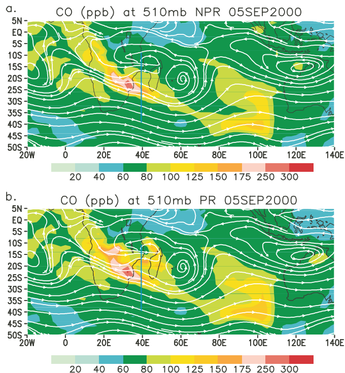
Fig. 11. Simulated CO concentrations for (a) the NPR run and (b) the PR run at 510 hPa in 5 September 2000. 3-day (3–5 September 2000) averaged streamlines in white are superimposed. The blue reference lines, used in Fig. 12, are drawn.
