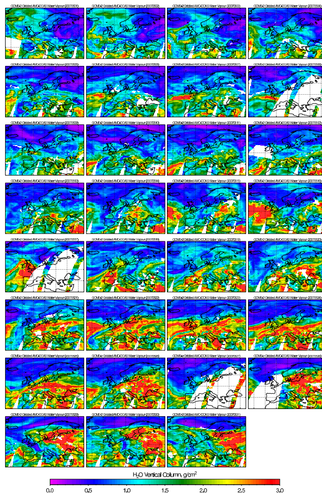
Fig. 6. GOME-2 daily water vapour data over Europe (gridded to 0.5^\circ \times 0.5^\circ in latitude/longitude) for May 2007.
