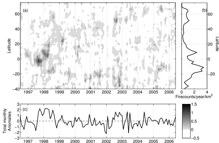
Fig. 1. (a) Time-latitude Hovmöller diagram of monthly deseasonalised fire anomalies (scale indicated by the colorbar). (b) Fire counts by latitude (detection/year/km 2 ), corrected by continental surface for each latitudinal band. (c) Monthly anomalies of the total deseasonalised fire counts over the 10 years.
