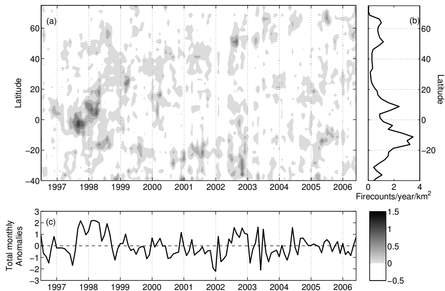
Fig. 1. (a) Time-latitude Hovmoller diagram of monthly deseasonalised fire anomalies (scale indicated by the colorbar). (b) Fire counts by latitude (detection/year/km 2 ), corrected by continental surface for each latitudinal band. (c) Monthly anomalies of the total deseasonalised fire counts over the 10 years.
