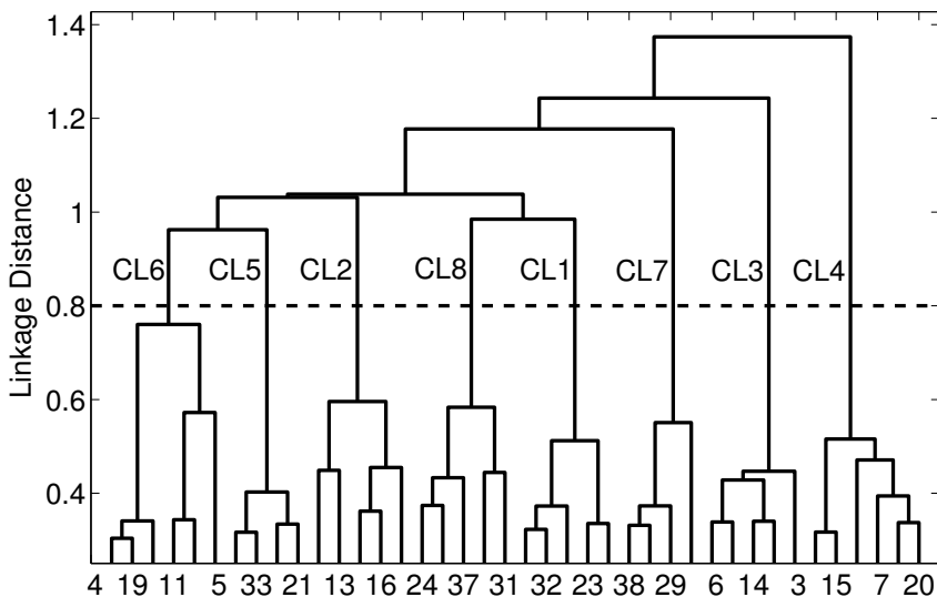
Fig. 6. Linkage distance tree. Retained clusters are indicated as CL#.
