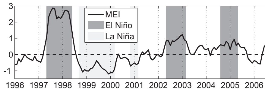
Fig. 2. MEI index time series. Darkgray/lightgray patches represent El Niño/La Niña as identified by the NOAA.
