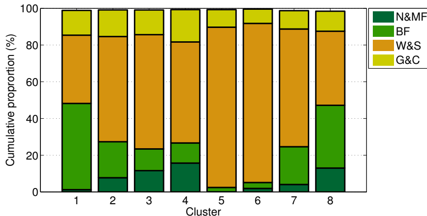
Fig. 10. Active fires incidence by landcover (UMD Landcover), for each cluster. N&MF: Needle-leaved and Mixed Forests; BF: Broadleaved Forests; W&S: Woodlands and Shrublands; G&C: Grasslands and Croplands.
