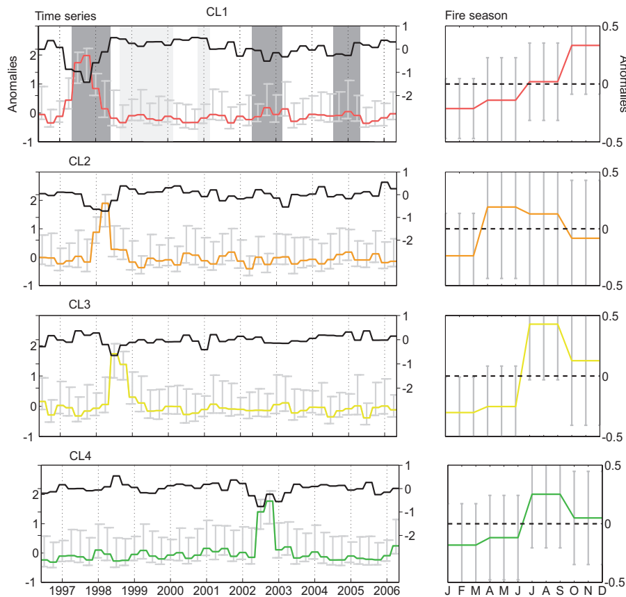
Fig. 9. (left) temporal profiles of fires (colored) and precipitation anomalies (CMAP data) and (right) averaged fire season.
