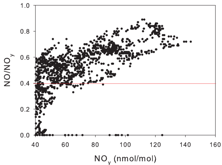
Fig. 15. Ratio of NO/NO y versus NO y for all data points with NO y >40 nmol/mol in winters 2004–2007.
