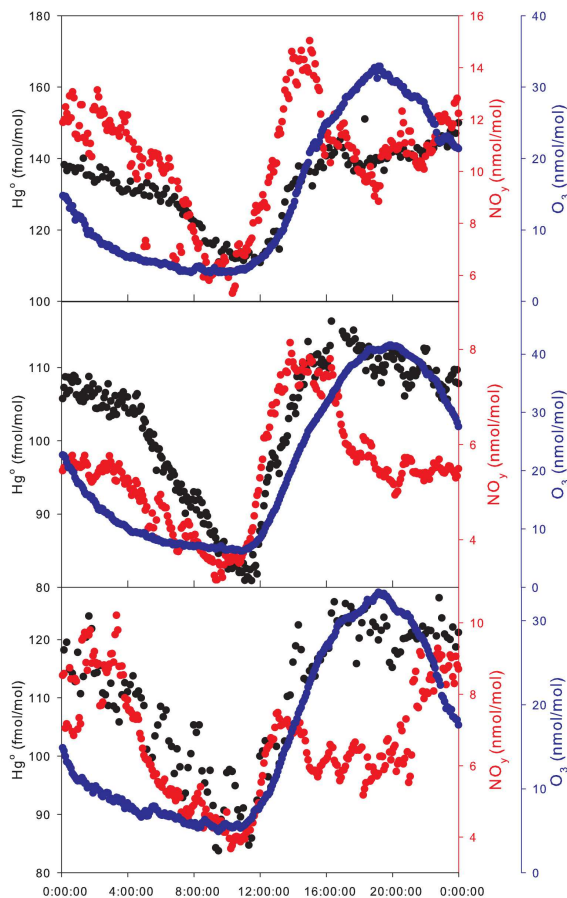
Fig. 10. Averaged diurnal cycles of Hg 0 (black), NO y (red), and O 3 (blue) for the days that include the data points with NO y < 40 nmol/mol on the lower boundary of Hg 0 vs. NO y presented in Fig. 9a.
