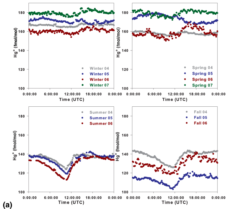
Fig. 2. Seasonally averaged diurnal cycles at TF (a) and PM (b) .
