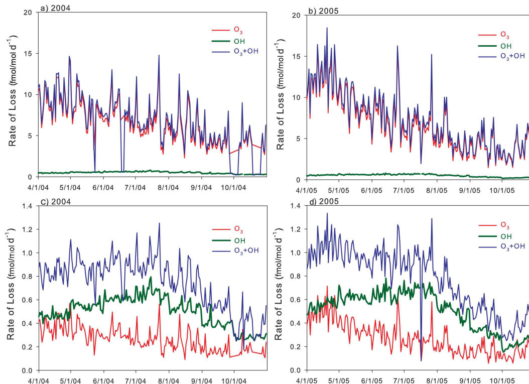
Fig. 8. Rate of loss of Hg 0 via oxidation reactions with O 3 (red), OH (green), and the total rate of loss during the warm season (1 April–31 October) in 2004 ( a , c ) and 2005 ( b , d ). The largest reaction rate constant 7.5 \times 10^{-19} \text{ cm}^3 \text{ molecule}^{-1} \text{ s}^{-1} (Calvert and Lindberg, 2005) was used in (a) and (b), and a constant on the lower end 3.0 \times 10^{-20} \text{ cm}^3 \text{ molecule}^{-1} \text{ s}^{-1} (Hall, 1995) was used in (c) and (d).
