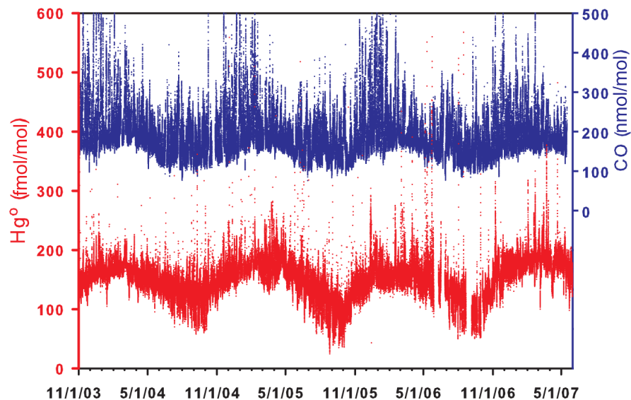
Fig. 3. Time series of 5-min averaged Hg ° (red) and CO (blue) at TF during the time period of 1 November 2003–31 May 2007.
