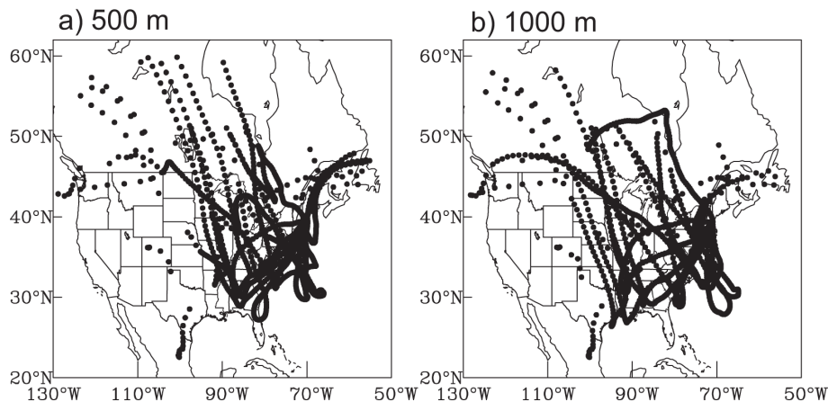
Fig. 14. Five-day backward trajectories using HYSPLIT for the 21 episodes of \text{NO}_y > 40 \text{ nmol/mol} in winters 2004–2007 starting at two heights, 500 m (a) and 1000 m (b) , at TF.
