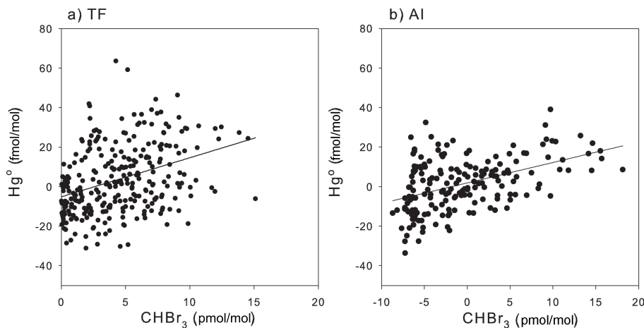
Fig. 11. Anomalies of Hg 0 versus CHBr 3 at TF (a) during summers 2004 and 2005 and at AI (b) in summer 2005. Anomalies were calculated by subtracting the hourly averages for the entire campaign period from the measured high resolution mixing ratios.
