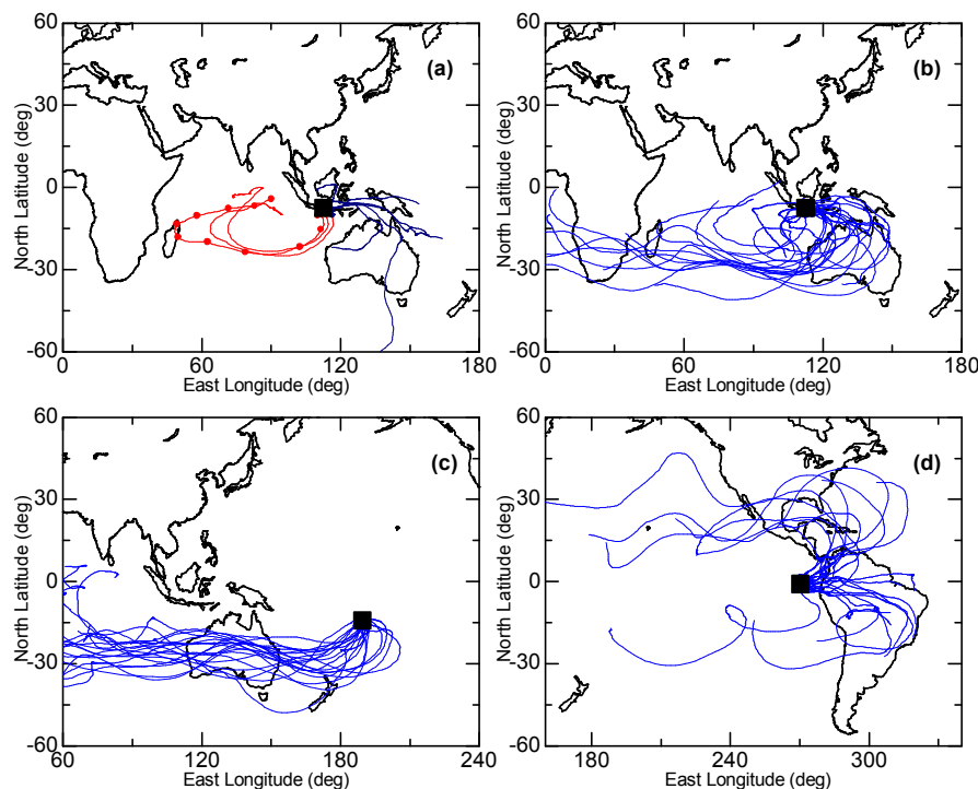
Fig. 9. Ten-day backward trajectories from the altitude of O_3 -enhanced layers with low relative humidity. (a) Trajectory from Watukosek on 7 June. Dots show the air mass position on a representative trajectory in each 24-h interval. (b) , (c) and (d) Twenty representative trajectories tracing back to the subtropical jet stream region from Watukosek, Samoa, and San Cristobal, respectively.
