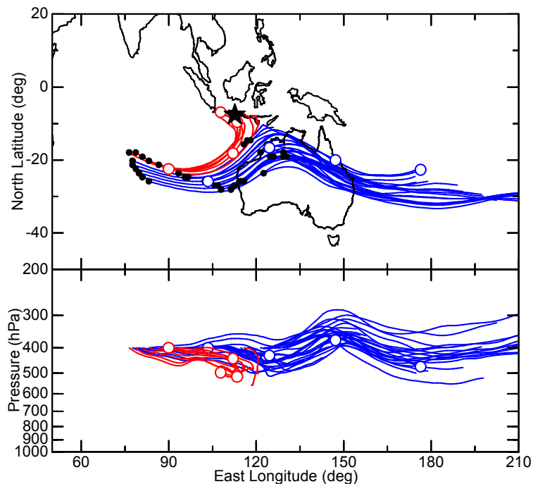
Fig. 11. Three-day forward trajectories calculated from the region of PV=-1 PVU shown in Fig. 10 on the 327K isentropic surface on 5 June 2000. White dots indicate the air mass position on representative trajectories in each 24-h interval.
