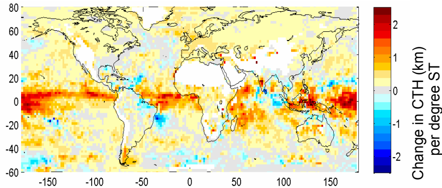
Fig. 10. Same as Fig. 8, but excluding the strong ENSO event (August 1997–July 1998). Even over the tropical oceans the differences compared to Fig. 8 are rather small.
