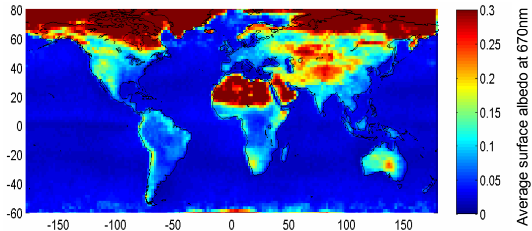
Fig. 4. Average surface albedo (670 nm) taken from Koелеmeijer et al. (2003).
