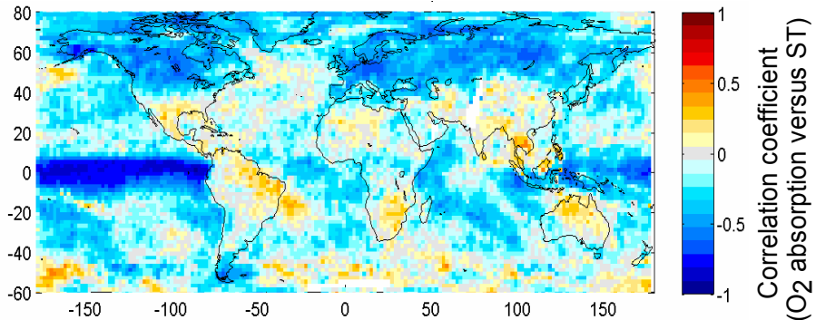
Fig. 7. Top: Correlation coefficients of the monthly anomalies of the effective cloud fraction versus surface-near temperature (top) and the O 2 absorption versus surface-near temperature (bottom).
