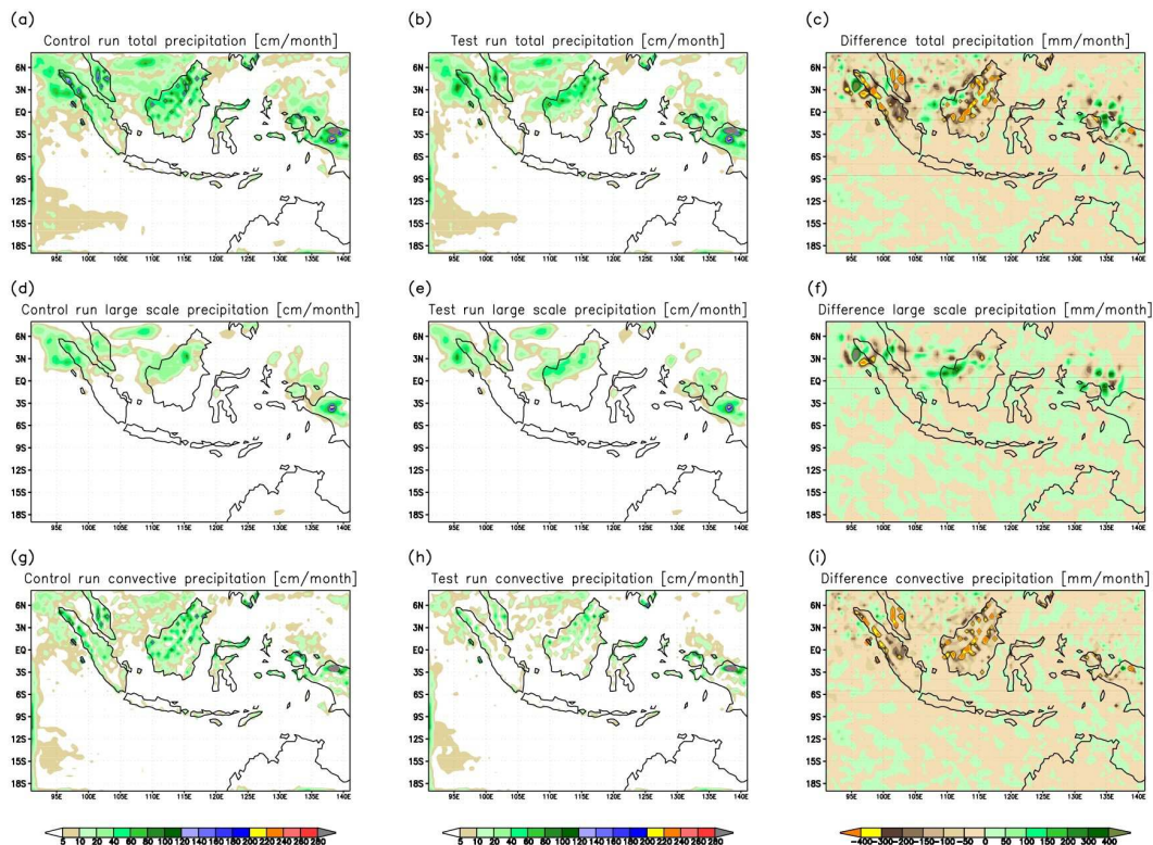
Fig. 2. Precipitation as simulated by REMOTE-CCFM simulated by REMOTE-CCFM and background CDNC (left column, total, large scale and convective rain from top to bottom), simulated by REMOTE-CCFM and background standard CDNC plus TPM (middle column) and precipitation anomalies between the two simulations (right column). Note that the colors for the differences (right column) are set to mm/month, while the absolute rainfall is in cm/month.
