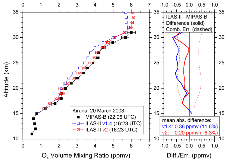
Fig. 1. Comparison of O_3 profiles measured by MIPAS-B and ILAS-II (data versions 1.4 (v1.4) and 2 (v2)) on 20 March 2003 above northern Scandinavia together with differences and combined total errors. Mean difference values are calculated over all coincident altitudes.
