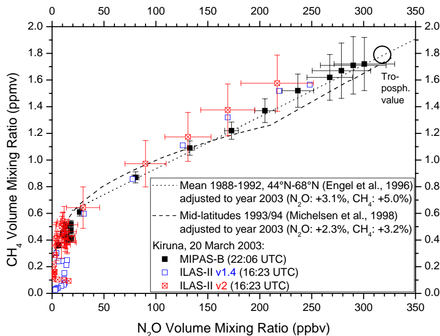
Fig. 4. N 2 O-CH 4 relationships as measured by MIPAS-B and ILAS-II (ILAS-II error bars for CH 4 values less than 0.3 ppmv are omitted for clarity). Trend-corrected reference correlations observed by other instruments (in-situ, Engel et al., 1996, and Atmospheric Trace Molecule Spectroscopy Experiment, Michelsen et al., 1998) are shown for comparison. The Northern Hemispheric tropospheric correlation value of 2003 is marked by a black circle.
