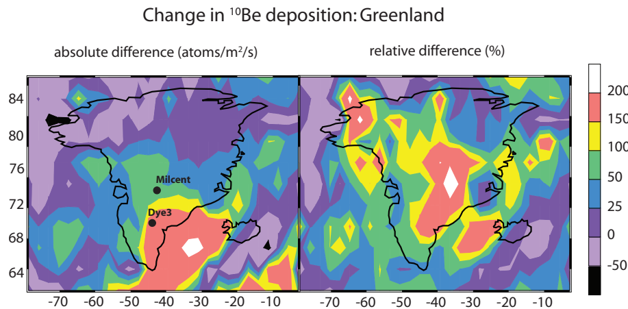
Fig. 8. The change of modeled ^{10}\text{Be} deposition between Maunder Minimum and Present Day in Greenland in absolute (atoms/m 2 /s, left) and relative (% , right) units.
