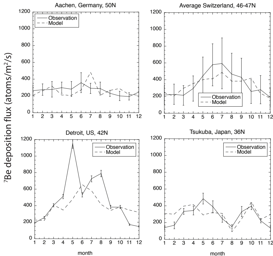
Fig. 4. ^7\text{Be} seasonal deposition fluxes modeled (dashed line) and observed (full line) in Germany, Switzerland, U.S. and Japan. The error bars show the standard deviations of the annual averages, except at Detroit, where the measurement errors (<5%) are shown. The observational data covers several years, except at Detroit (18 months).
