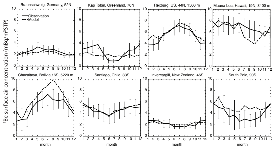
Fig. 3. Seasonal cycles of ^7\text{Be} measured (full line) in surface air ( \text{mBq/m}^3\text{STP} ) at selected stations worldwide compared with the modeled (dashed line) concentrations. The error bars show the standard deviations of the monthly averages of the different years (8–30 years depending on the station).
