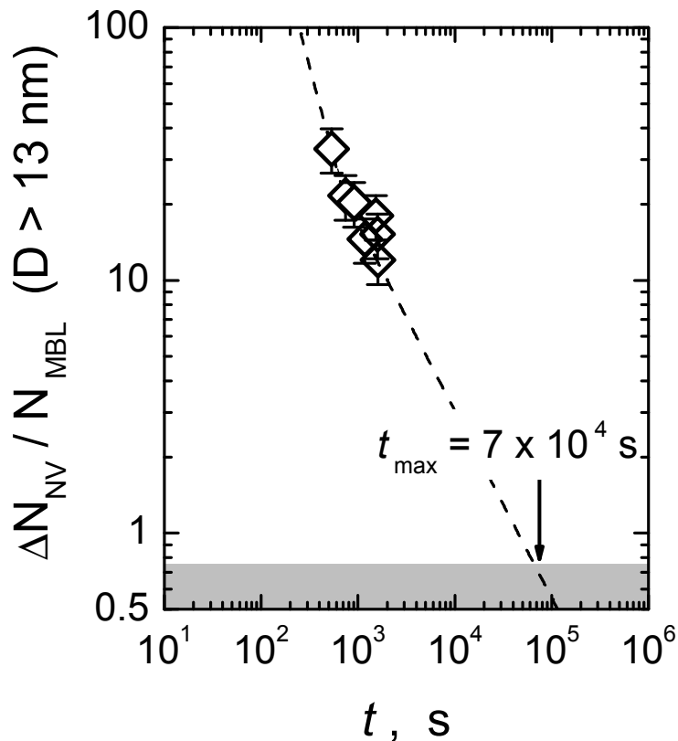
Fig. 14. Ship plume particle signature in terms of excess non-volatile particles in the plume per marine BL particles as a function of plume age t ; the maximum detectable plume age of 7 \times 10^4 \text{ s} corresponds to the plume age for which the plume signal becomes indistinguishable from a varying MBL aerosol.
