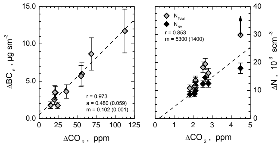
Fig. 10. Emission factors derived from the MAERSK vessel plume: BC_e from near field data with BC_e > LOD ; N_{NV} from far field data with N_{NV} below the CPC coincidence level of 20\,000 cm^{-3} . Intercept a , slope m , and correlation coefficient r of the regression lines are added to the panels (uncertainties in parentheses).
