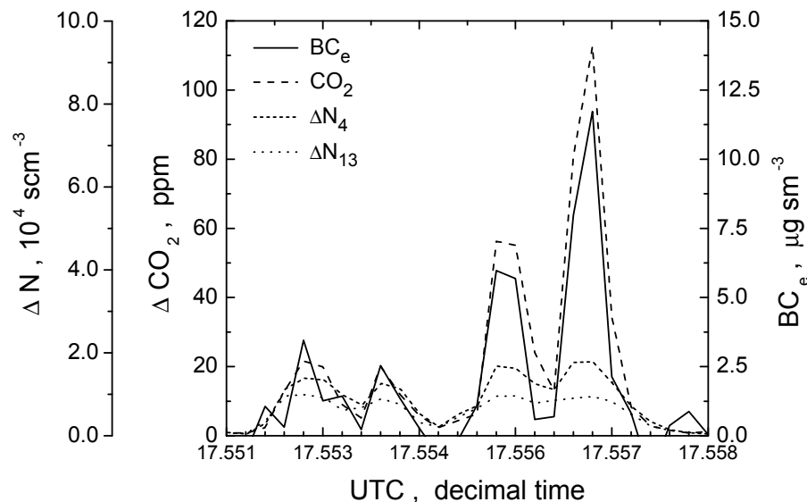
Fig. 8. Raw data of the closest plume encounter: equivalent black carbon from aerosol light absorption measurement ( BC_e ; solid line), excess CO_2 ( \Delta CO_2 : dashed line), and excess number densities of particles with D > 4 nm ( \Delta N_4 : short dotted line) and D > 13 nm ( \Delta N_{13} : dotted line).
