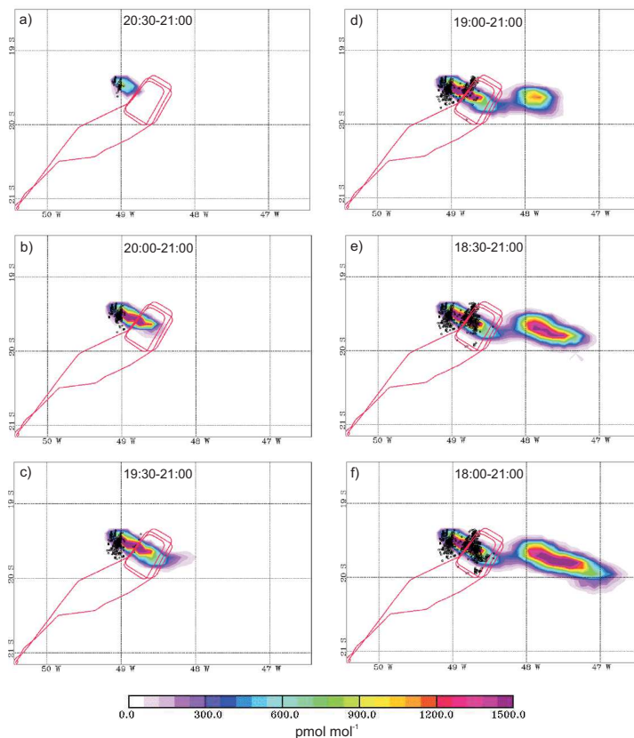
Fig. 7. FLEXPART lightning tracer simulations (NO x at 10 km in pmol mol -1 ) for the 18 February 2005 subtropical thunderstorm system considering all LINET strokes (black dots) after (a) 20:30 UTC, (b) 20:00 UTC, (c) 19:30 UTC, (d) 19:00 UTC, (e) 18:30 UTC, (f) 18:00 UTC and until 21:00 UTC. The Falcon track is superimposed in red.
