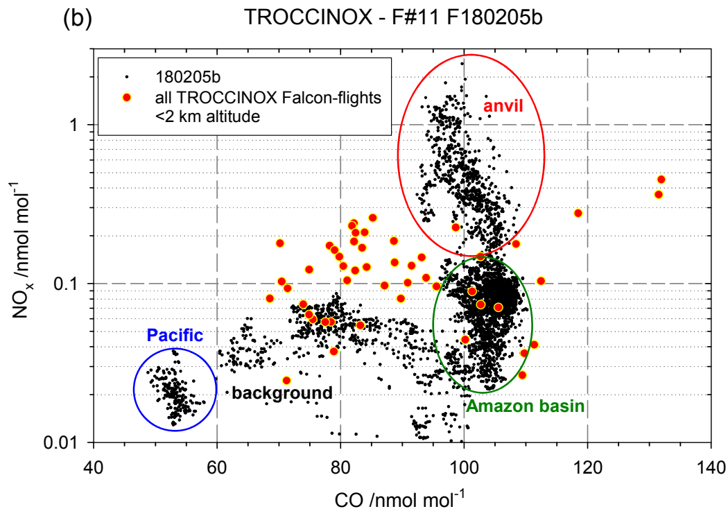
Fig. 10b. (b) Correlation plot for \text{NO}_x and CO for the same flight (black dots), and superimposed data from all TROCCINOX Falcon-flights in the boundary layer (<2 km) (red-yellow dots).
