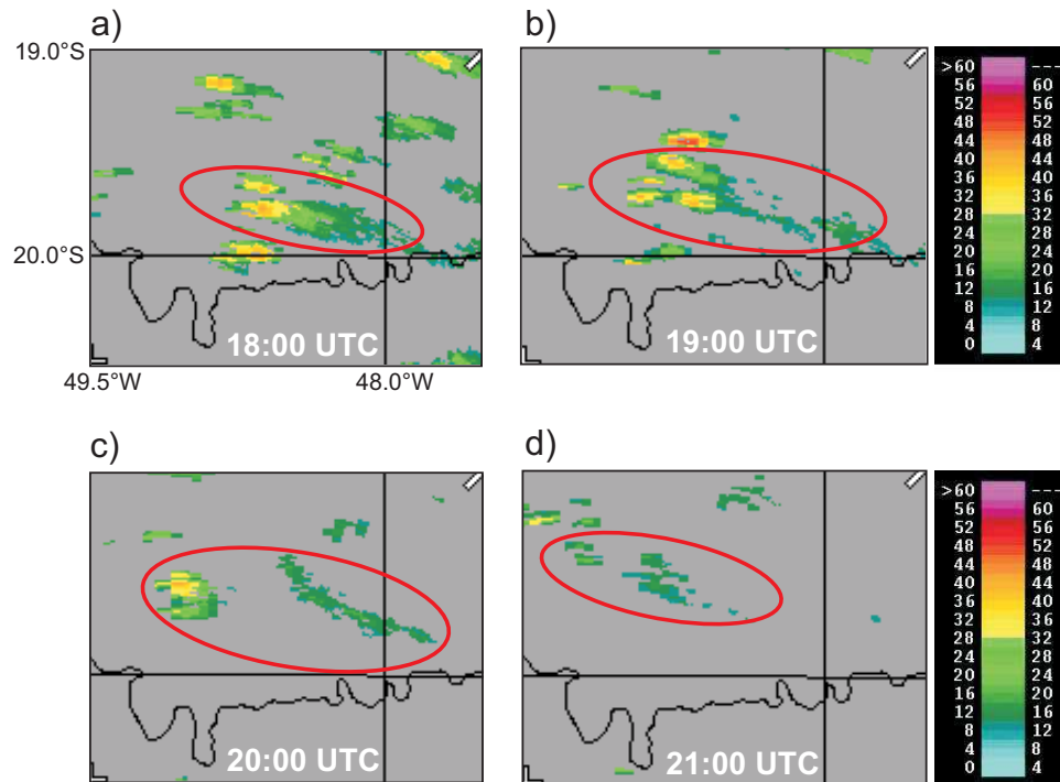
Fig. 8. Radar reflectivity as PPI scan (PPI_SURVEILLANCE operational product) in dBZ units measured at 0.0° elevation by the Bauru radar (22.4° S, 49.0° W) for the 18 February 2005 sub-tropical thunderstorm system (marked in red) at (a) 18:00 UTC, (b) 19:00 UTC, (c) 20:00 UTC and (d) 21:00 UTC.
