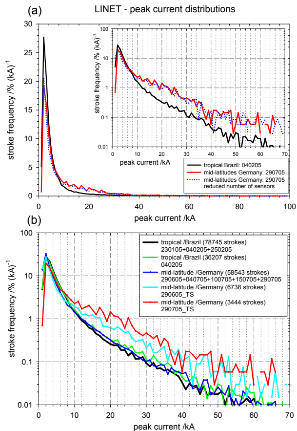
Fig. 17. Frequency distributions of LINET strokes (in the LINET centre area) as a function of peak current for different datasets given in colour (for comparison all curves were normalised). (c) Estimated amount of NO produced per 1 kA stroke interval (based on the Wang et al. 1998 relationship) for the dataset in (a) considering different values for C_{\text{LINET}} .
