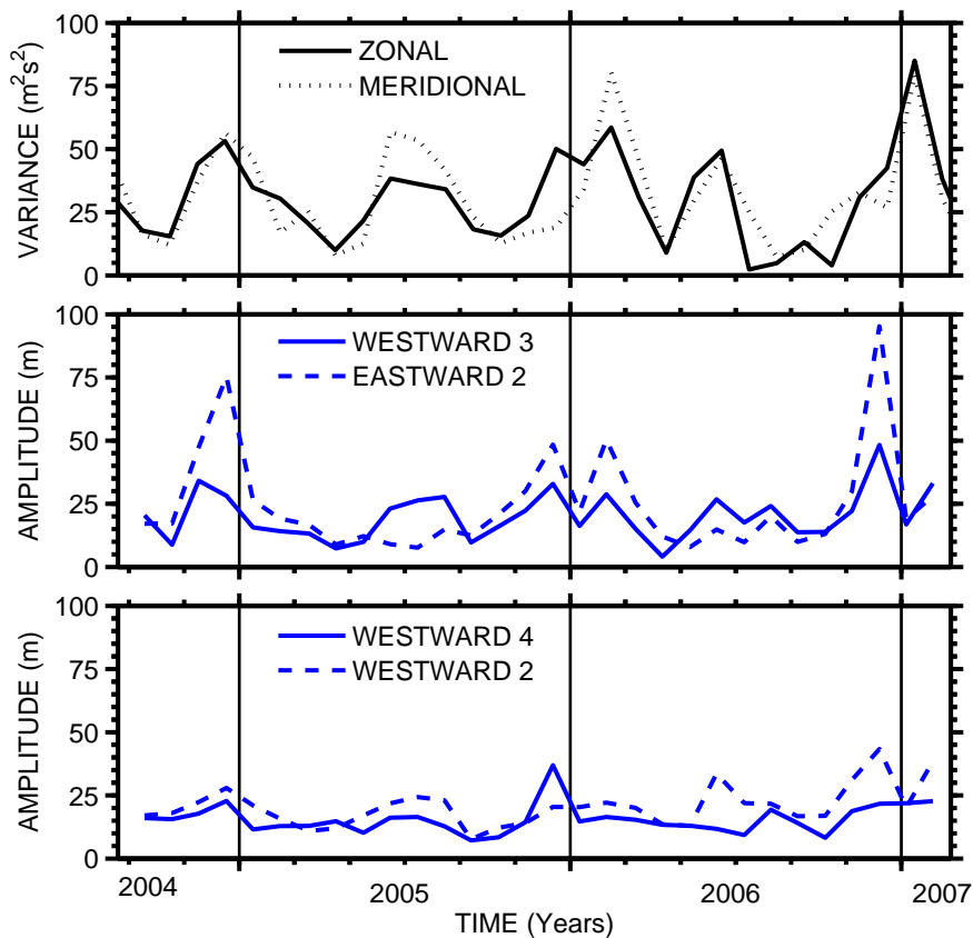
Fig. 4. (a) Horizontal wind variances from the Esrange meteor radar for a height of 89–92 km as per Fig. 1. (b) Geopotential height amplitudes at a height of \sim 91 km, between 63^\circ and 73^\circ N, over the period range 42 to 56 h for W3 and E2. (c) as (b) but for W4 and W2.
