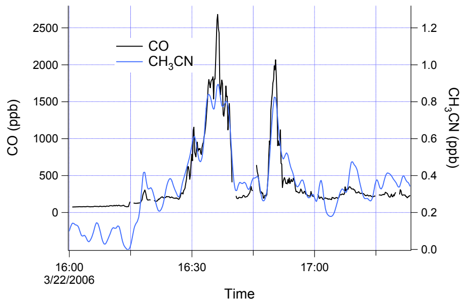
Fig. 5. Time series in UTC for CO and CH 3 CN on flight 322a. Urban plume was encountered on L4 (16:35) and then L0 (16:50). Linear least squares regression for urban plume, excluding points with high CH 3 CN according to Eq. (2) gave \text{CO} = 105 + 21.9 \text{ NO}_y , r^2 = 0.97 . The CO and CH 3 CN axes are scaled by \text{CH}_3\text{CN} = 0.2 + 0.4 \times 10^{-3} \text{ CO} which describes the proportionality between CH 3 CN and CO in the urban plume. Points where the CH 3 CN (blue) curve are above the CO (black) curve are identified as having a significant biomass burning influence.
