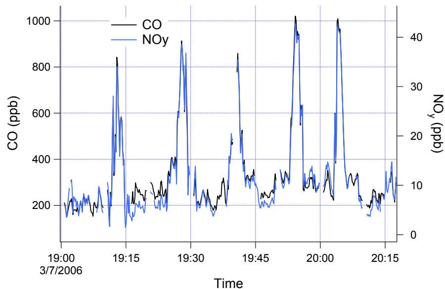
Fig. 3. Time series in UTC for CO and NO y on flight 307a containing 5 passes through the urban plume encountered on Legs 4 and 5. Proportionality between CO and NO y causes CO trace to be largely hidden by NO y trace during plume passages.
