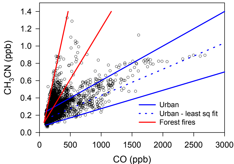
Fig. 4. Scatter plot of CH 3 CN vs. CO concentration. Each data point is a 10 s measurement period which satisfies criteria in Table 4 except for the limits on CH 3 CN and on (CO-100)/NO y . Red lines encompass the range of CH 3 CN – CO relations found in forest fire plumes by de Gouw et al. (2006). Blue lines encompass data points designated as having an urban source of CH 3 CN. Bottom blue line is an approximate indication of the lower limit of CH 3 CN in urban samples. Data points above the top blue line, given by Eq. (2), are eliminated from subsequent analysis as having a significant forest fire influence.
