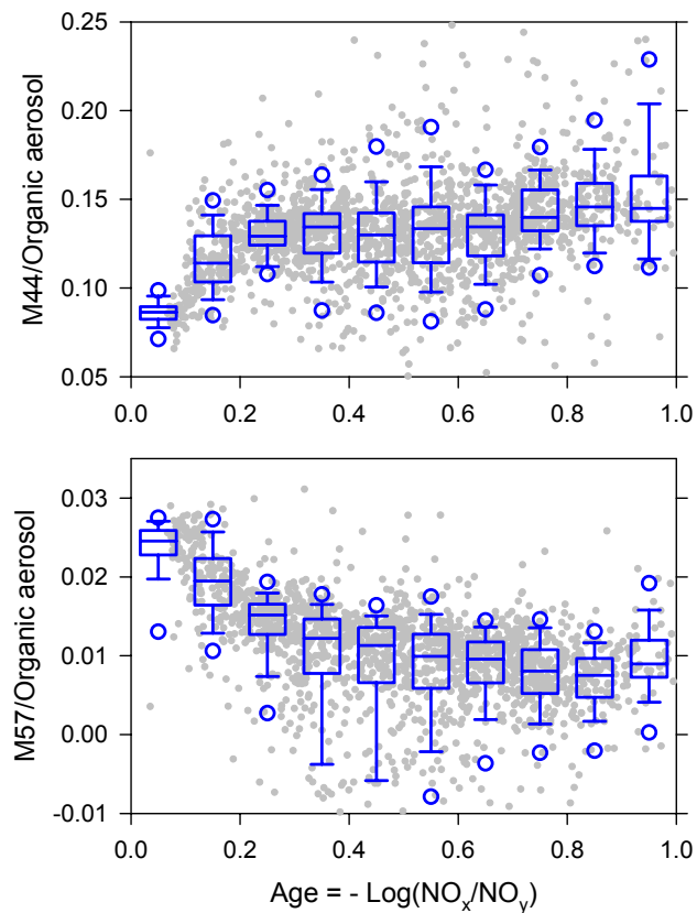
Fig. 12. Fraction of organic aerosol mass that is (a) M44 ( \text{amu}/z=44 ) and (b) M57 ( \text{amu}/z=57 ). Box plots have same format as Fig. 8.
