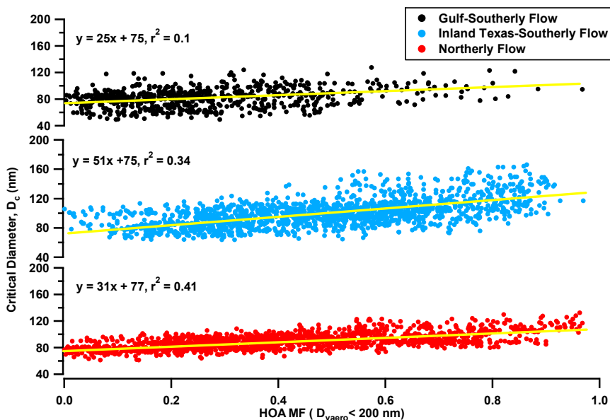
Fig. 5. HOA mass fraction of the AMS mass for the size range D_{\text{vaero}} < 200 \text{ nm} vs. critical diameter calculated at 0.44% supersaturation. Shown are the data from the three wind-radon regimes.
