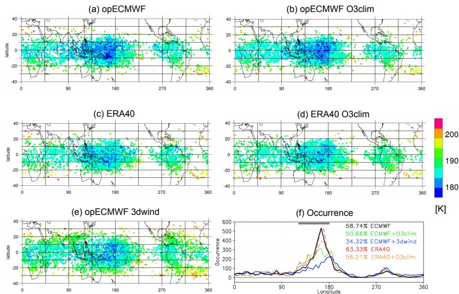
Fig. 1. Maps of LCP temperature [K] during DJF 2001/2002 for (a) opECMWF heating rates (black line in f), (b) opECMWF heating rates derived from climatological ozone (green line in f), (c) ERA40 heating rates (red line in f), (d) ERA40 heating rates derived from climatological ozone (orange line in f), (e) opECMWF vertical wind (blue line in f). Each square marks one trajectory. (f) Occurrence of LCP trajectories averaged over 40° S–40° N, inside 5° longitude bins. The numbers in % indicate the percent of trajectories traveling through the 120° E–180° E region.
