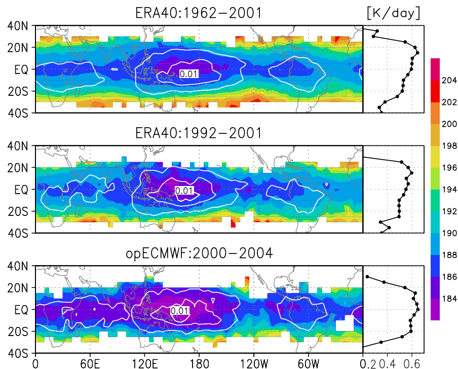
Fig. 3. DJF long-term climatology; Left: LCP temperature [K] (color) and the density of LCPs (white contours); Right: Zonal mean \bar{Q}_{LCP} [K/day]. Top panel: 1962/1963–2001/2002 ERA40 data; middle panel: 1992/1993–2001/2002 ERA40 data; lower panel: opECMWF data from 2000/2001–2004/2005. Contour intervals for the density are 0.001, 0.005 and 0.01 per 5^\circ \times 5^\circ grid.
