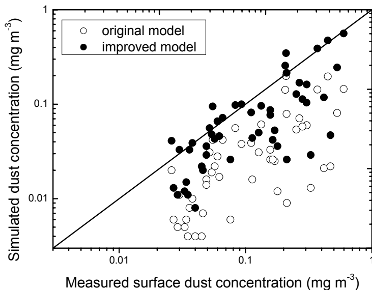
Fig. 6. A comparison of monthly mean surface dust concentration between measurements at Asian sites and corresponding model results. Data, locations and time period are listed in Table 4. Solid line is the 1 to 1 line. Logarithm scale is used in order to show some low values of model results. Correlation coefficients of original and improved models are 0.56 and 0.71 respectively.
