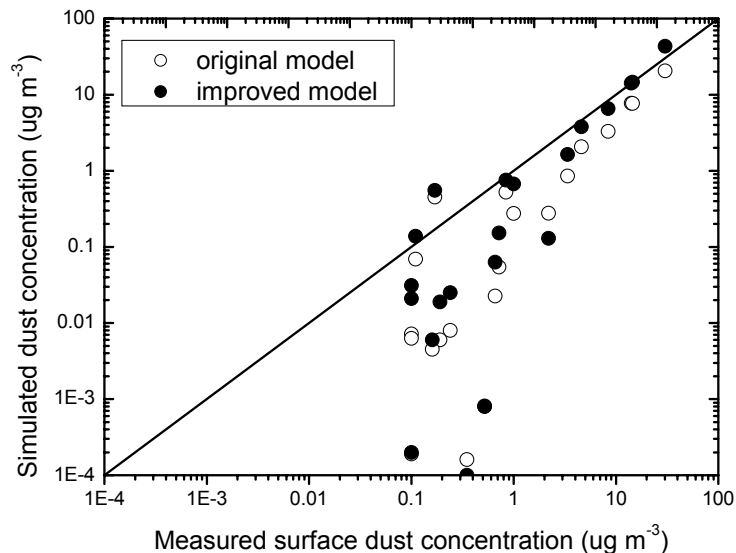
Fig. 4. A comparison of annual mean surface dust concentration between measurements at remote marine sites and corresponding model results. Data and site locations are listed in Table 3. Solid line is the 1 to 1 line. Logarithm scale is used in order to show some low values of model results. Correlation coefficients of original and improved models are 0.98 and 0.99 respectively.
