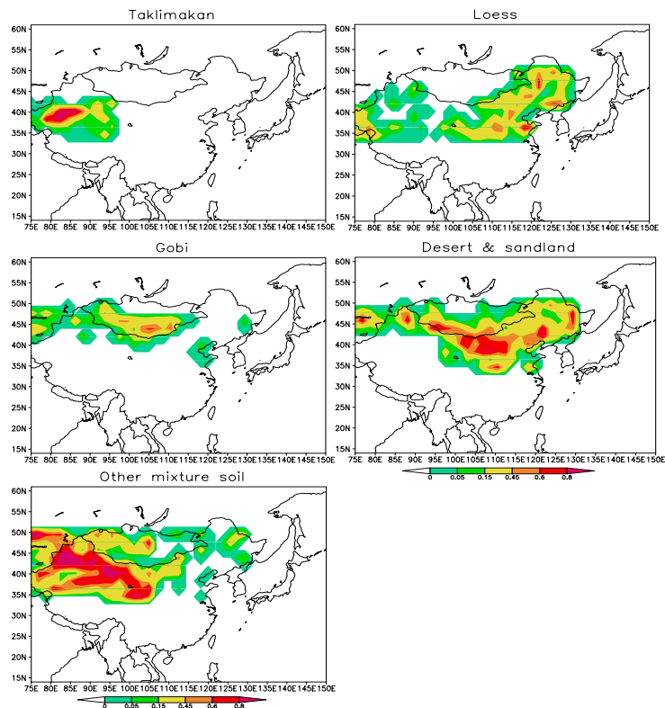
Fig. 2. Area percentages of 5 updated soil types in East-Asian dust source areas with a horizontal resolution of 1.8^\circ \times 1.8^\circ .
