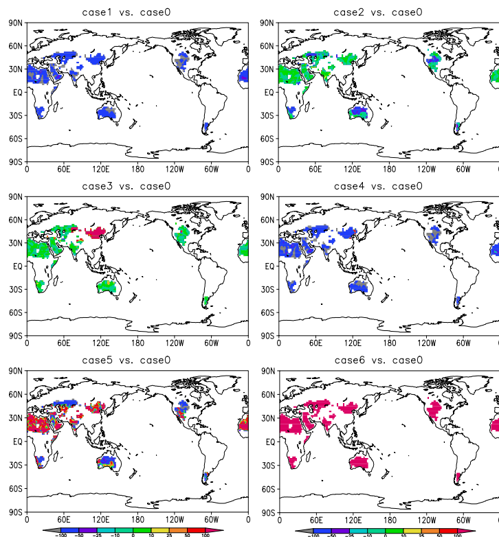
Fig. 3. Percentage differences (%) between sensitivity simulations and the reference simulation in terms of the annual mean dust emission amount ( \text{Tgyr}^{-1} , global mean values are listed in column 6 of Table 2).
