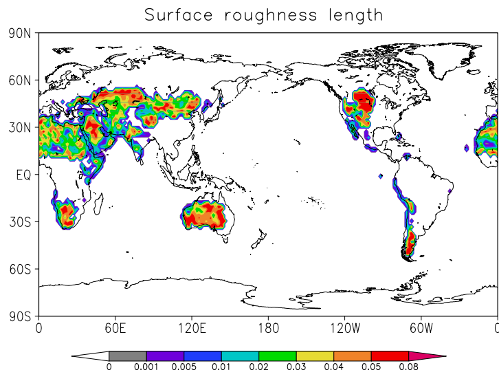
Fig. 1. Updated annual mean field of aerodynamic surface roughness length Z_0 (cm) with a horizontal resolution of 1.8^\circ \times 1.8^\circ (Prigent et al., 2005). Data are shown only in arid and semi-arid areas of the globe, forests and dense vegetated regions are excluded because they are not potential dust source areas.
