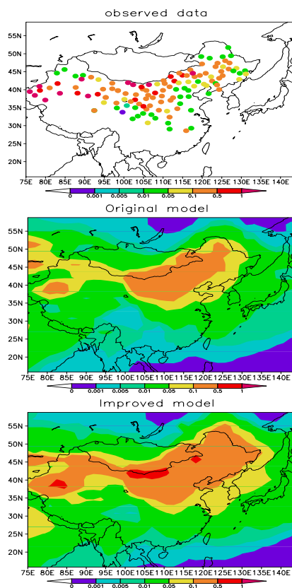
Fig. 5. A comparison of monthly mean surface dust concentration ( \text{mg m}^{-3} ) in East Asia for April, 2001. The observed data are derived from visibility. Dust concentrations between 0.001 and 1 \text{ mg m}^{-3} as indicated in the color bar are corresponding to visibilities of 69.2, 54.7, 48.4, 33.8, 27.5, 12.8 and 6.5 km respectively (Shao et al., 2003). Model results are taken from simulations with the original and improved dust emission scheme (case 0 and case 5) respectively.
